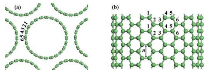
FIG. 4. (Color online) (a) Arrangement of the atoms in a (12, 12) nanotube, showing the six representative atoms. (b) Periodicity of atomic pairs along the tube axis. n = 0.2425 nm.
