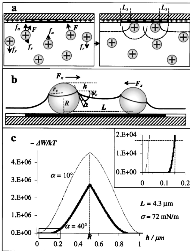
FIG. 4. Schematic presentation of the two-stage mechanism of colloidal assembly on a \mu -patterned ionic substrate (see text for details). (a) Specific deposition driven by screened Coulomb interactions. (b) Focusing of the structure due to lateral capillary attraction (adopted from [5]). (c) Energy of capillary interaction as a function of the receding of the liquid layer.
