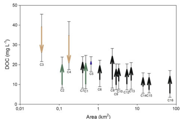
Figure 2. Average variability in DOC concentration for the 15 catchments from baseflow to high flow (2003–2008). The tail and head of arrows are average baseflow (<0.15 mm day -1 ) and high flow (>5.5 mm day -1 ) concentrations, respectively. The whiskers denote the standard deviation of average concentrations. Light brown arrows are wetland-dominated catchments (C3 and C4), green arrows are the forest-dominated catchments (C1 and C2), and blue arrow is the lake outlet (C5), whereas the black arrows denote mixed catchments (Color figure online).
