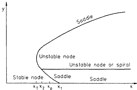
Fig. 12. Bifurcation diagram 3
