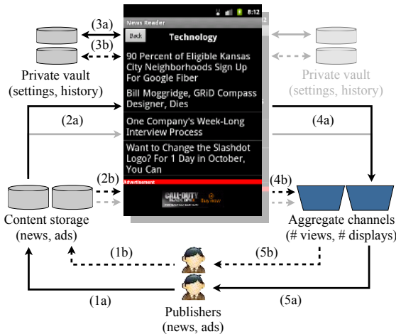
FIGURE 9—Interactions and data flow between the news reader app and \pi Box. The dark (solid, dotted) lines represent the flow from the (content, ad) publisher. The lighter lines represent the same flows for another user of the same app.
