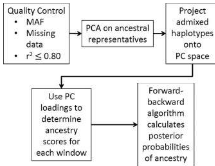
Figure 1. Outline of the PCAdmix algorithm.
