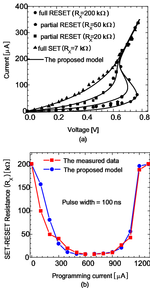
Fig. 4. (a) I-V comparison between the measured data [1] and the proposed unified model [6], (b) Comparison between the measured data [1] and simulated resistance in the full SET, full RESET, partial SET, and partial RESET state [6].
