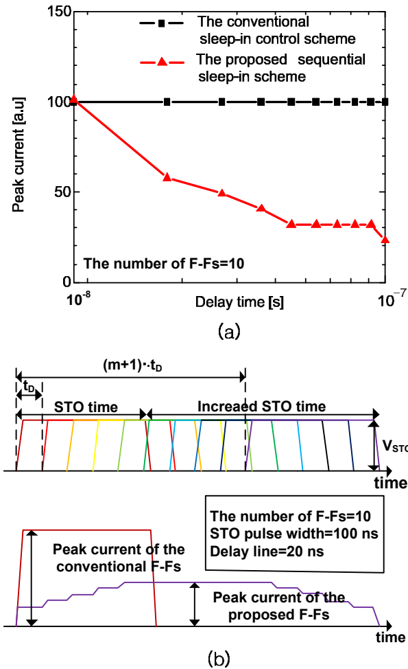
Fig. 7. (a) Comparison of peak current between the conventional sleep-in control scheme and the proposed sequential sleep-in scheme, (b) Peak current reduction of the proposed scheme.
