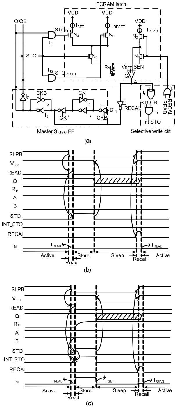
Fig. 2. (a) FF-2 circuit with selective write latch, (b) the timing diagram of FF-2 when the FF-2's data is the same with the stored data at PCRAM latch, (c) the timing diagram of FF-2 when the FF-2's data is different from the stored data at the PCRAM latch.
