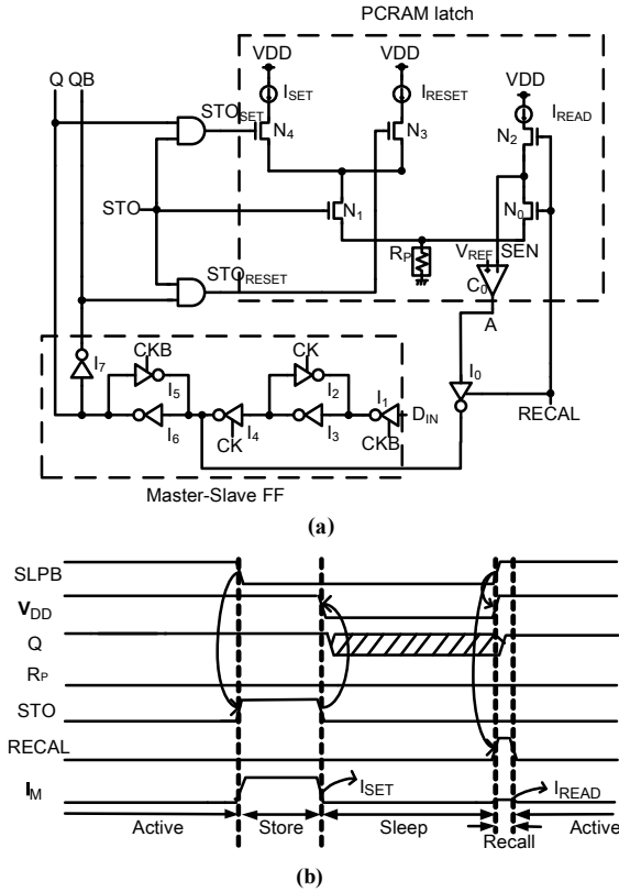
Fig. 1. (a) FF-1 circuit with PCRAM latch, (b) its timing diagram.
