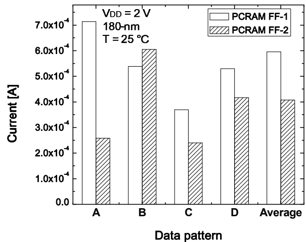
Fig. 5. Current consumption of the FF-1 and FF-2 circuits in the storing operation for various data patterns. The data patterns for A, B, C, and D are ‘000000’, 101010’, ‘111111’, and ‘11001100’, respectively. Here I_{SET} and I_{RESET} are 600 \mu\text{A} and 1250 \mu\text{A} , respectively. The cycle time for the STORE and RECALL operation is 370 ns.
