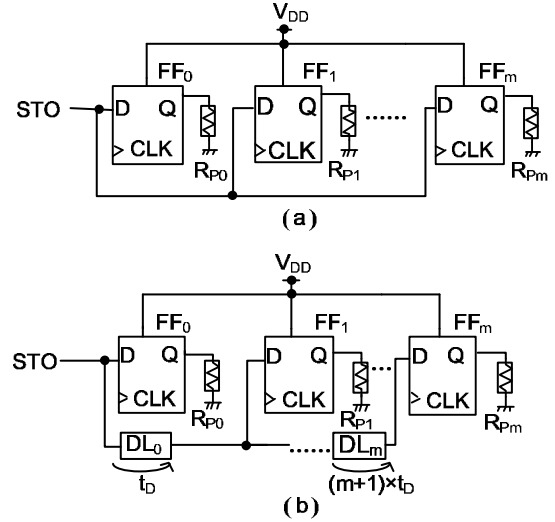
Fig. 3. (a) The conventional sleep-in control scheme, (b) the proposed sequential sleep-in control scheme. DL means the delay line.
