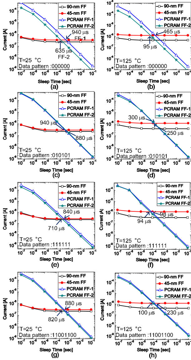
Fig. 6. Comparison of current dissipation between the conventional FFs with 45-nm and 90-nm, the FF-1, and the FF-2. Here the crossover times of FF-1 and FF-2 whose sleep energies are equal to the conventional 45-nm FF are written inside these figures. The crossover times of FF-1 and FF-2 are shown in right and left, respectively (a) Data pattern=000000, T=25\text{ }^{\circ}\text{C} , (b) Data pattern=000000, T=125\text{ }^{\circ}\text{C} , (c) Data pattern=010101, T=25\text{ }^{\circ}\text{C} , (d) Data pattern=010101, T=125\text{ }^{\circ}\text{C} , (e) Data pattern=111111, T=25\text{ }^{\circ}\text{C} , (f) Data pattern=111111, T=125\text{ }^{\circ}\text{C} , (g) Data pattern=11001100, T=25\text{ }^{\circ}\text{C} , (h) Data pattern=11001100, T=125\text{ }^{\circ}\text{C} .
