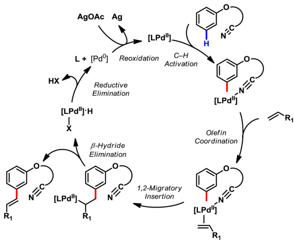
Figure 4. Catalytic Cycle of meta -C-H Olefination
