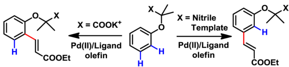
Figure 2. Remote ortho - and meta -C-H Functionalizations
