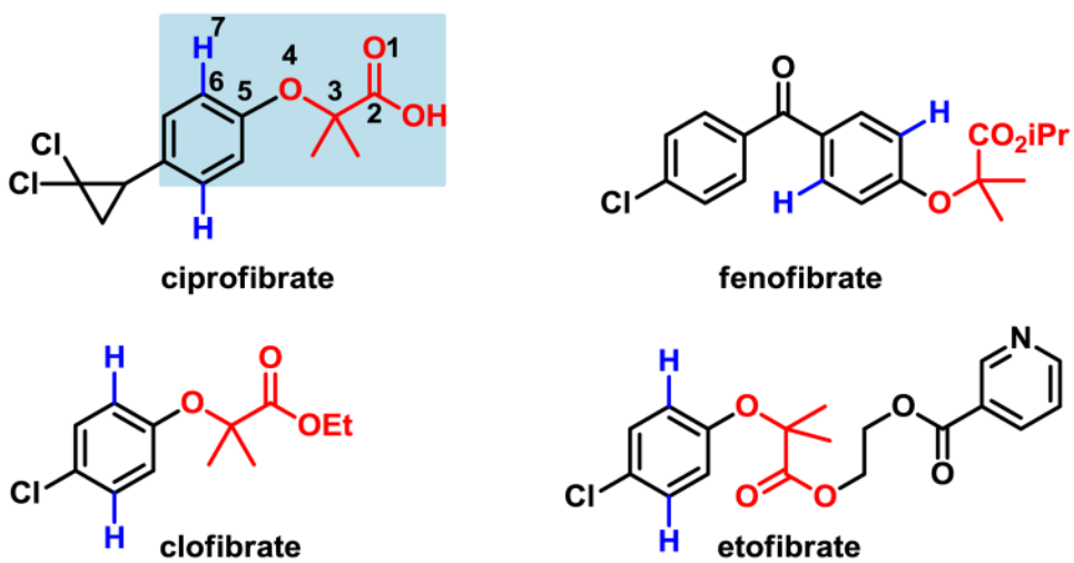
Figure 3. Drug Molecules Based on \alpha -Phenoxyacetic Acids
