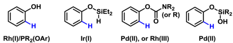
Figure 1. Previous ortho -C–H Functionalizations of Phenol
