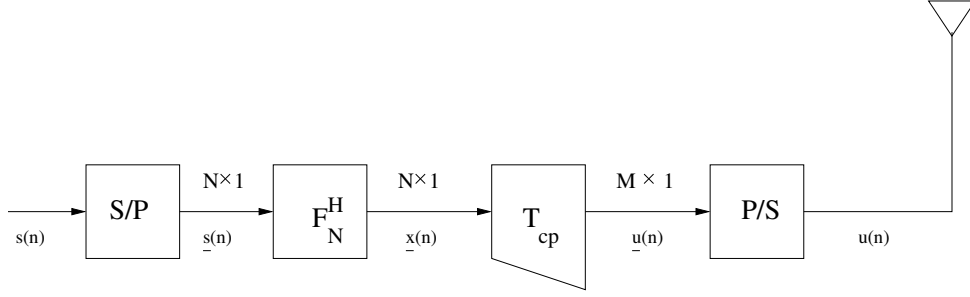
Figure 2.1: OFDM Transmitter
