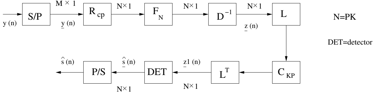
Figure 4.9: Matrix model for IOFDM receiver
