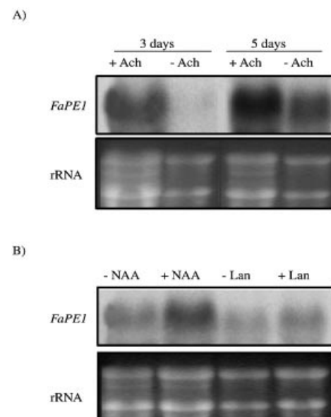
Fig. 4. Effect of auxins on FaPE1 expression. Northern blot analysis of total RNA (15 \mu g) extracted from green fruits under different auxin conditions. (A) FaPE1 expression in the presence (+Ach) or absence (-Ach) of achenes 3 d and 5 d after deaenation. (B) FaPE1 expression in untreated (-NAA) and 3 d after the application of 1 mM NAA in a lanolin paste (+NAA). As a control for the auxin treatment, another set of fruits were treated with the lanolin paste only (+Lan) or left untreated (-Lan).
