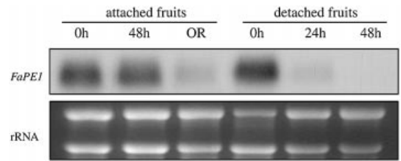
Fig. 6. Northern blot analysis of FaPE1 expression during senescence of strawberry fruit whilst either detached or attached to their parent plant. Attached fruit were allowed to senesce until overripe (OR), whilst detached fruit were allowed to ripen for 48 h.
