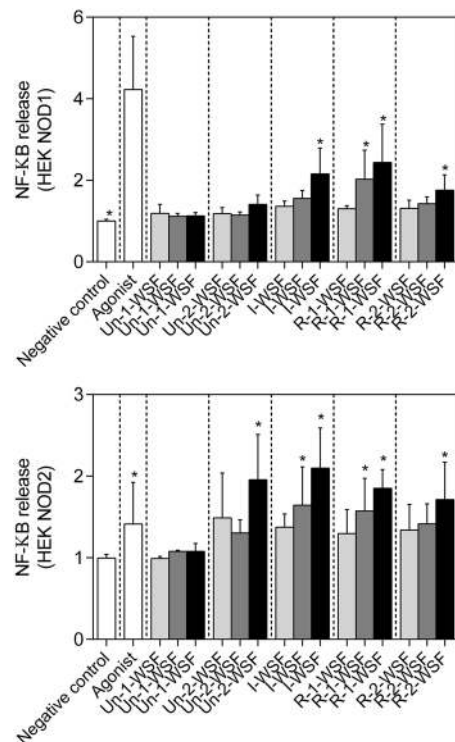
Figure 5. NOD1 and NOD2 reporter cells NF- \kappa B/AP-1 activation after papaya pectin treatments. Un-1-WSF: unripe - papaya from 1 st day after harvest - water-soluble fraction; Un-2-WSF: unripe - papaya from 2 nd day after harvest - water-soluble fraction; I-WSF: intermediate ripening time point - papaya from 3 rd day after harvest - water-soluble fraction; R-1-WSF: ripe - papaya from 4 th day after harvest - water-soluble fraction; R-2-WSF: ripe - papaya from 5 th day after harvest - water-soluble fraction. According Dunnett's * p value < 0.05 when compared with negative control.
