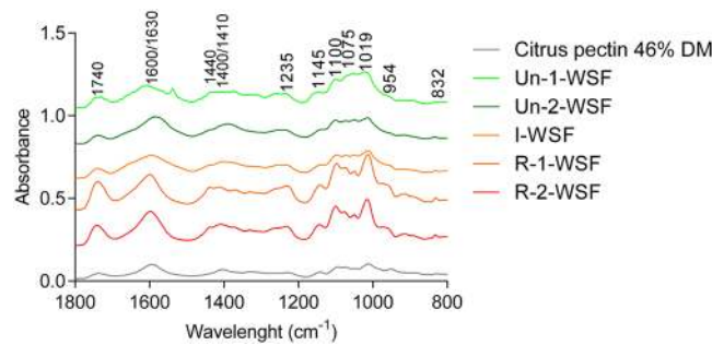
Figure 3. FT-IR spectra of citrus pectin DM 46% and papayas water-soluble fraction (WSF). Un-1-WSF: unripe - papaya from 1 st day after harvest - water-soluble fraction; Un-2-WSF: unripe - papaya from 2 nd day after harvest - water-soluble fraction; I-WSF: intermediate ripening time point - papaya from 3 rd day after harvest - water-soluble fraction; R-1-WSF: ripe - papaya from 4 th day after harvest - water-soluble fraction; R-2-WSF: ripe - papaya from 5 th day after harvest - water-soluble fraction.
