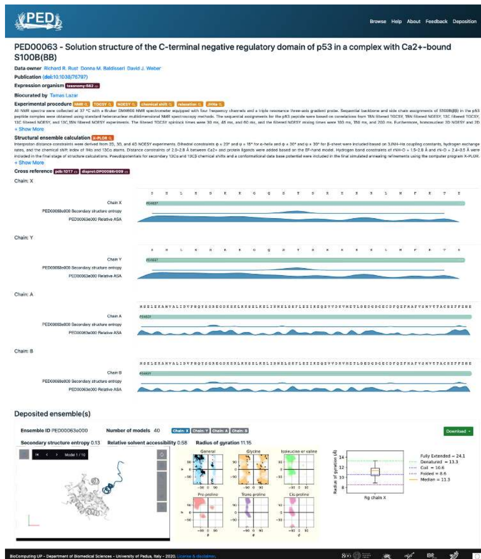
Figure 4. Example for PED's Entry page. Entry page is shown for the C-terminal disordered region of p53 in a tetrameric complex with \text{Ca}^{2+} -bound S100B (PED00063). The feature view shows chain-specific information, while molecular graphics, Ramachandran maps and R_g distribution are presented below.
