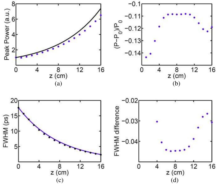
Figure 3.12: Evolution of (a) peak power (b) peak power difference (c) FWHM and (d) FWHM difference along grating length. The physical parameters are same as that of the dots in Fig. 3.11 when b = 2 . The solid curve and dots represent the self-similar solution, and the results of NLCM simulation, respectively.
