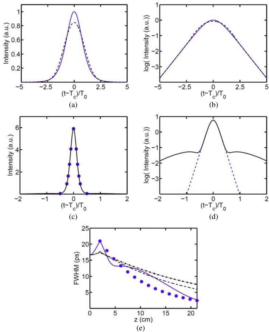
Figure 2.7: Hyperbolic secant input pulse. The pulse profiles before (solid curve) and after the linear FBG (dashed curve) in (a) linear and (b) logarithmic scales. The pulse profiles after the NFBG (solid curve) and a “fitted” hyperbolic secant pulse profiles in (c) linear (dots) and (d) logarithmic scales (dashed curve). (e) Evolution of the FWHM in the pre-chirper (the linear FBG) and the NFBG for the self-similar soliton (dots), the full numerical simulation (solid curve), the LVM using hyperbolic secant pulse ansatz (dashed curve), and the POM using hyperbolic secant pulse ansatz (dot-dashed curve).
