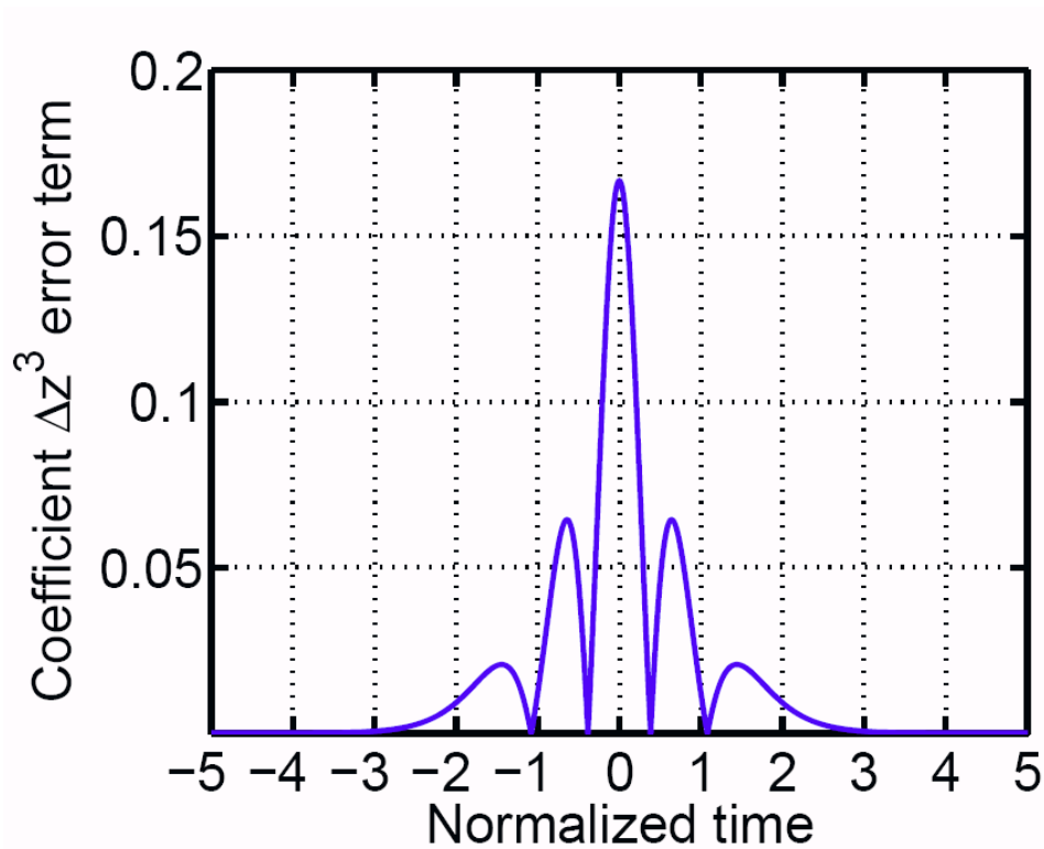
Figure E.1: The coefficient leading order (\Delta z)^3 error term in a symmetrized split-step Fourier algorithm. The simple soliton solution q(z, t) = \text{sech}(t)\exp(iz/2) is used.
