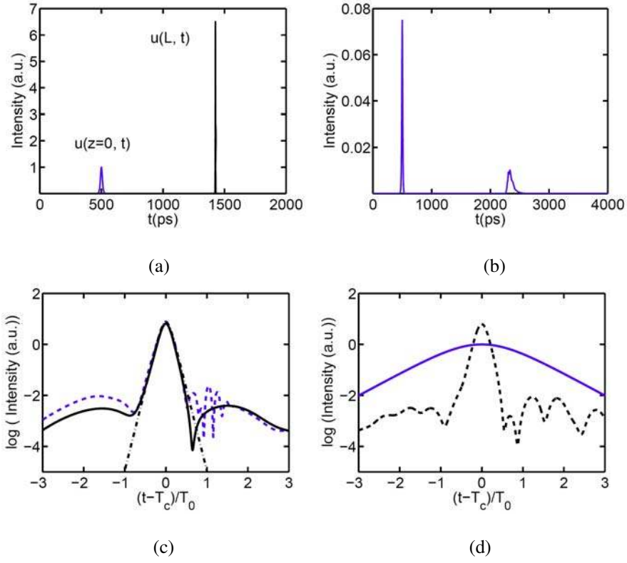
Figure 3.1: Chirped hyperbolic secant pulse is the initial pulse. (a) Launched pulse u(z=0,t) and transmitted pulse u(L,t) . (b) Reflected pulse v(z=0,t) . (c) Transmitted pulse (solid curve: NLCMEs; dashed curve: NLSE with \beta_3 ; dot-dashed curve: NLSE without \beta_3 ) in logarithmic scale. (d) Initial (solid curve) and transmitted pulse (dashed curve) in 8-section SWA. Discussion on Fig. 3.1 (d) will be offered in Section 3.3.3. The grating parameters are \beta_{20} = -25 \text{ ps}^2/\text{cm} , \sigma = 0.125 \text{ /cm} , b = 2 , \gamma = 5 \text{ /W/km} , and L = 16 \text{ cm} .
