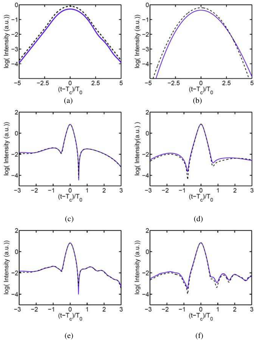
Figure 3.18: Pre-chirped pulse when (a) chirp-free hyperbolic secant pulse or (b) chirp-free Gaussian pulse is the initial pulse. Compressed pulses when (c) chirp-free hyperbolic secant pulse or (d) chirp-free Gaussian pulse is the initial pulse. (e) Compressed pulse in 8-section SWA of Fig. 3.18(c). (f) Compressed pulse in 8-section SWA of Fig. 3.18(d). Solid curve: linear grating is the prechirper. Dashed curve: linear fiber is the prechirper.
