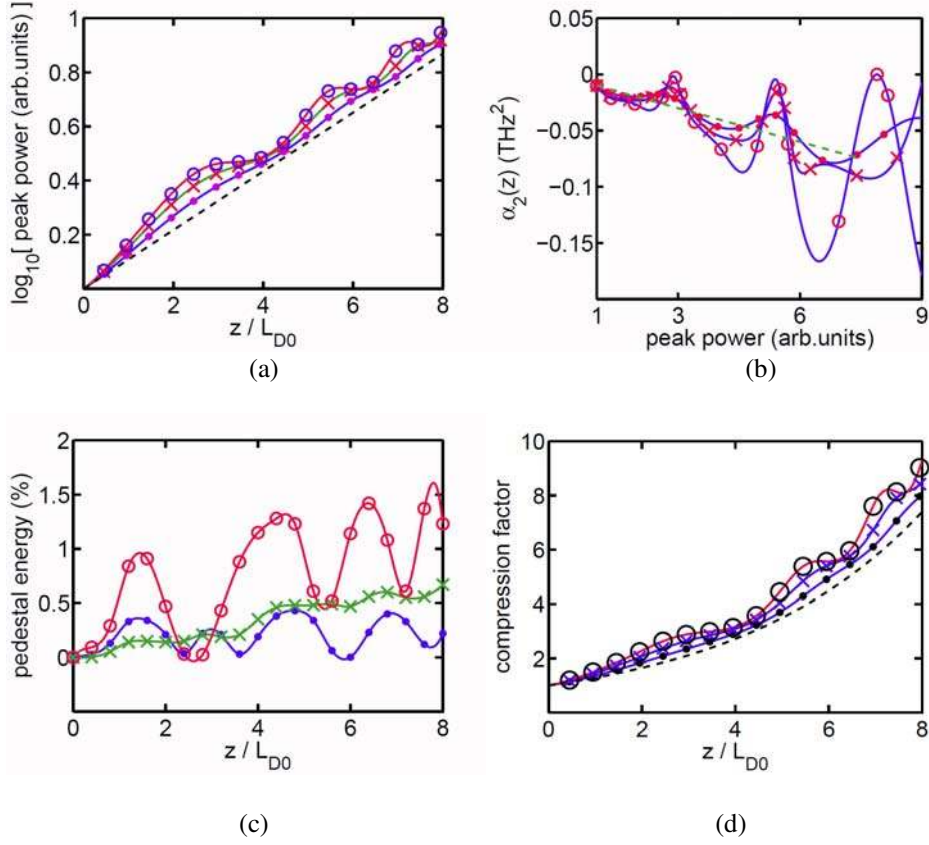
Figure 4.4: Evolution of the (a) peak power, (b) chirp, (c) pedestal energy, and (d) compression factor when the initial peak power deviates +20% from the ideal peak power when distance varies from 0 to 400 m for the same physical parameters used in Fig 4.1. The parameter L_{D0} is the initial dispersion length. The dashed curve represents results for the exact solution, dots represent results for competing cubic-quintic nonlinearities ( \delta_0 = 0.4724 / W^2/m ), circles represent results for cooperating cubic-quintic nonlinearities ( \delta_0 = -0.4724 / W^2/m ), and crosses represent results for pure cubic nonlinearity ( \delta_0 = 0 ).
