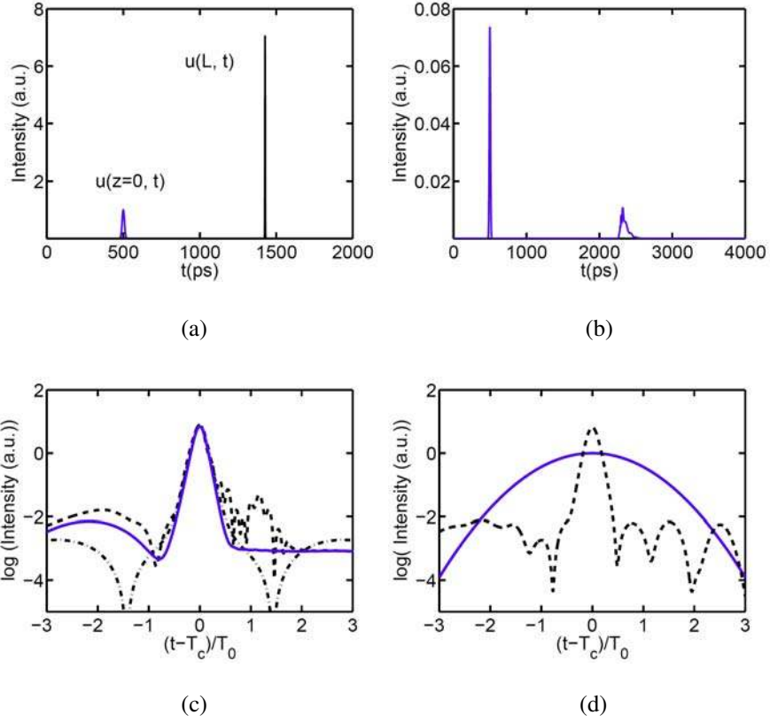
Figure 3.2: Chirped Gaussian pulse is the initial pulse. (a) Launched pulse u(z=0,t) and transmitted pulse u(L,t) . (b) Reflected pulse v(z=0,t) . (c) Initial pulse (dots) and transmitted pulse (solid curve: NLCMEs; dashed curve: NLSE with \beta_3 ; dot-dashed curve: NLSE without \beta_3 ) in logarithmic scale. (d) Initial pulse (solid curve) and compressed pulse (dashed curve) in 8-section SWA. Discussion on Fig. 3.2(d) will be offered in Section 3.3.3. The grating parameters are \beta_{20} = -25 \text{ ps}^2/\text{cm} , \sigma = 0.125 \text{ /cm} , b = 2 , \gamma = 5 \text{ /W/km} , and L = 16 \text{ cm} .
