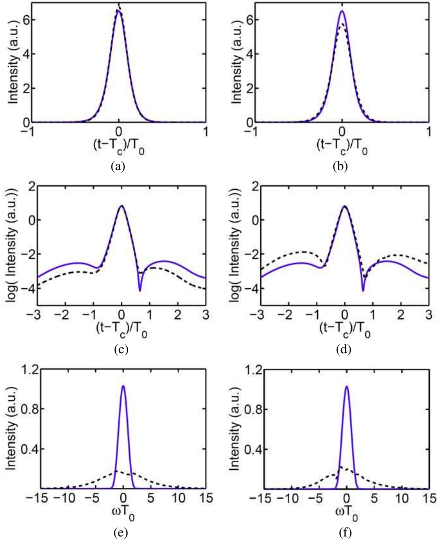
Figure 3.16: Chirped hyperbolic secant pulse ( \text{sech}(t/T_0) \exp(i\alpha_{20}t^2/2) , \alpha_{20} = -0.005 \text{ THz}^2 , T_0 = 10 \text{ ps} ) is the initial pulse. Compressed pulse in (a) linear and (c) logarithmic scale where the physical parameters for the dashed curve are \beta_{20} = -12.5 \text{ ps}^2/\text{cm} , b = 2 , \gamma = 5 \text{ /W/km} , L = 32 \text{ cm} . Compressed pulse in (b) linear and (d) logarithmic scale where the physical parameters for the dashed curve are \beta_{20} = -50 \text{ ps}^2/\text{cm} , b = 2 , \gamma = 5 \text{ /W/km} , L = 8 \text{ cm} . The solid curve in (a, b, c, d) corresponds to the compressed pulse in Fig. 3.1. (e) Spectra of initial pulse (solid curve) and compressed pulse (dashed curve) for Fig. 3.16(a). (f) Spectra of initial pulse (solid curve) and compressed pulse (dashed curve) for Fig. 3.16(b).
