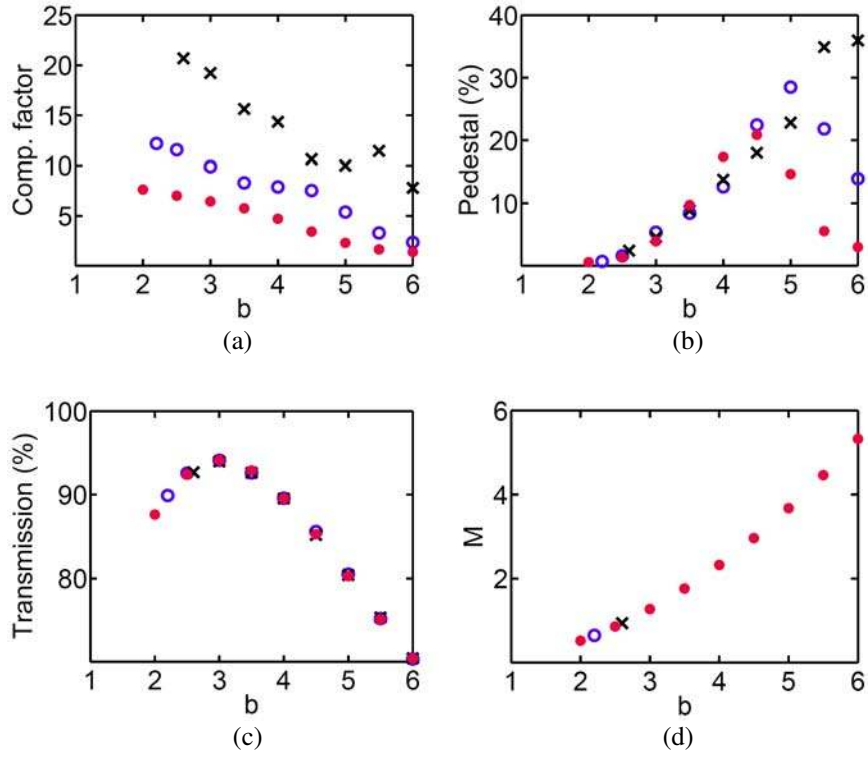
Figure 3.11: (a) Compression factor (b) pedestal (c) transmission (d) M versus b . The initial pulse is \text{sech}(t/T_0)\exp(i\alpha_{20}t^2/2) , where T_0 = 10 ps, \alpha_{20} = -0.005 THz 2 . The grating parameters are \beta_{20} = -25 ps 2 /cm, \sigma = 0.125 /cm, \gamma = 5 /W/km, L = 16 cm (dots), 20 cm (circles), and 25 cm (crosses). For L = 16 cm, b = 2, 2.5, 3, 3.5, 4, 4.5, 5, 5.5, 6 . For L = 20 cm, b = 2.2, 2.5, 3, 3.5, 4, 4.5, 5, 5.5, 6 . For L = 25 cm, b = 2.6, 3, 3.5, 4, 4.5, 5, 5.5, 6 .
