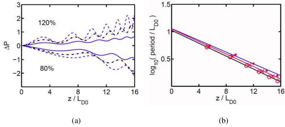
Figure 4.5: (a) Evolution of \Delta P = P_{\text{perturbed}} - P_{\text{ideal}} along the propagation direction. The solid curve represents results for competing cubic-quintic nonlinearities ( \delta_0 = 0.4724 / \text{W}^2/\text{m} ), dashed curve represents results for cooperating cubic-quintic nonlinearities ( \delta_0 = -0.4724 / \text{W}^2/\text{m} ), dot-dashed curve represents results for pure cubic nonlinearity ( \delta_0 = 0 ). The physical parameters are T_0 = 5 ps, \alpha_{20} = -0.005 THz 2 , \beta_0 = -0.5 ps 2 /m, \sigma = 0.0025 /m, \gamma_0 = 0.2362 /W/m, g = 0 and z = 800 m. (b) Variation of the oscillation periods along the propagation direction. The dots represent results for competing cubic-quintic nonlinearities ( \delta_0 = 0.4724/\text{W}^2/\text{m} ), circles represent results for cooperating cubic-quintic nonlinearities ( \delta_0 = -0.4724/\text{W}^2/\text{m} ), crosses represent results for pure cubic nonlinearity ( \delta_0 = 0 ). The solid curve represents exponential fittings for the three different cases.
