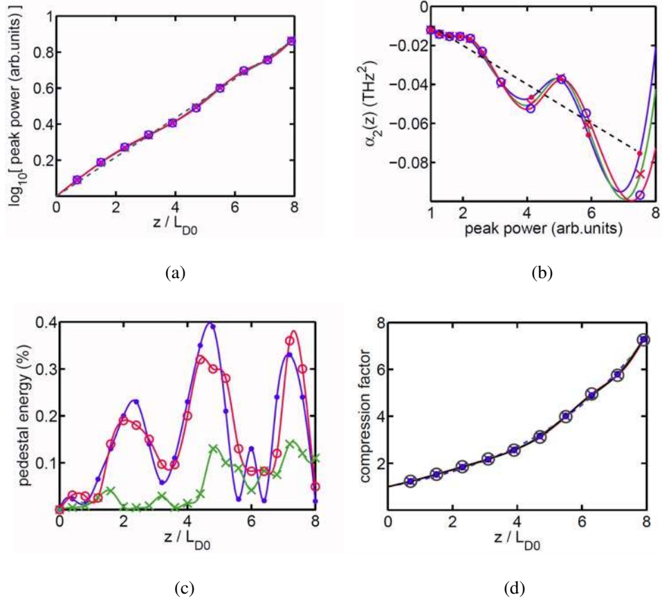
Figure 4.7: Evolution of the (a) peak power, (b) chirp, (c) pedestal energy, and (d) compression factor when the initial chirp deviates +20% from the exact chirp when the distance varies from 0 to 400 m for the same physical parameters in Fig 4.1. The dashed curve represents results for the exact solution, dots represent results for competing cubic- quintic nonlinearities ( \delta_0 = 0.4724 \text{ /W}^2\text{/m} ), circles represent results for cooperating cubic- quintic nonlinearities ( \delta_0 = -0.4724 \text{ /W}^2\text{/m} ), and crosses represent results for pure cubic nonlinearity ( \delta_0 = 0 ).
