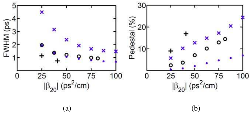
Figure 3.19: (a) FWHM (ps) and (b) pedestal (%) of the compressed pulse versus different initial dispersion. Dots: b = 2 , T_0 = 10 ps, \alpha_{20} = -0.005 THz 2 , \varepsilon = 2 ; circles: b = 2 , T_0 = 10 ps, \alpha_{20} = -0.01 THz 2 , \varepsilon = 1 ; crosses: b = 2 , T_0 = 20 ps, \alpha_{20} = -0.005 THz 2 , \varepsilon = 0.5 ; plus signs: b = 2 , T_0 = 5 ps, \alpha_{20} = -0.04 THz 2 , \varepsilon = 1 .
