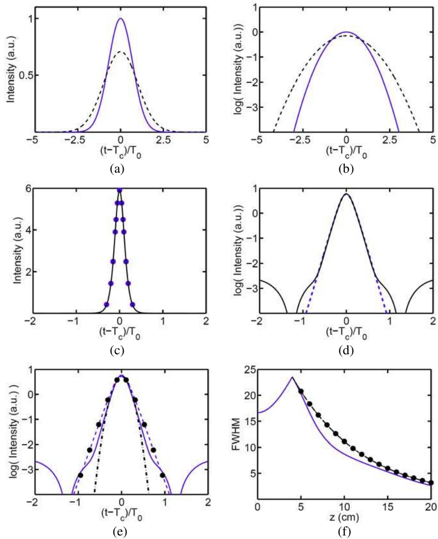
Figure 2.8: Gaussian input pulse. The pulse profiles before (solid curve) and after the linear FBG (dashed curve) in (a) linear and (b) logarithmic scales. The pulse profiles after the NFBG (solid curve) and a “fitted” hyperbolic secant pulse profiles in (c) linear (dots) and (d) logarithmic scales (dashed curve). (e) The compressed pulse in logarithmic scale. (f) Evolution of the FWHM in pre-chirper (linear FBG) and the NFBG. For (e) and (f), the solid curve, dashed curve, dots, and dot-dashed curve represent the full numerical simulation, the LVM with hyperbolic secant pulse ansatz, the POM with hyperbolic secant pulse ansatz, and the LVM or POM with Gaussian ansatz, respectively.
