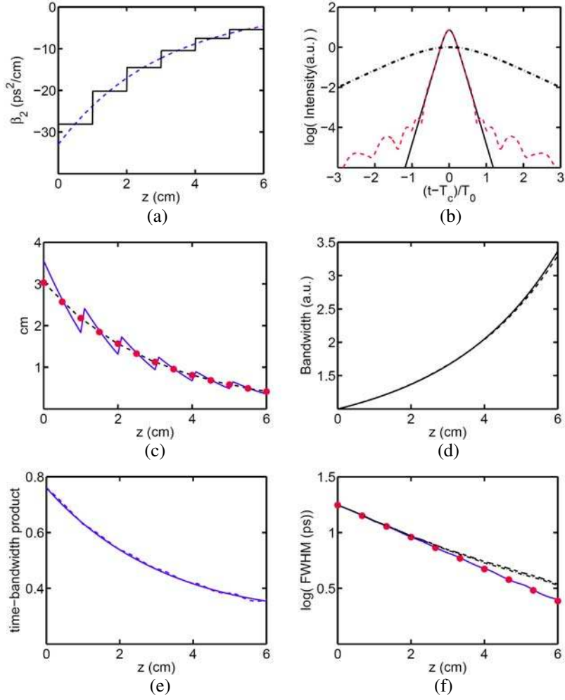
Figure 2.4: The exponentially decreasing dispersion profile (dashed curve) and the 6-section SWA (solid curve). (b) The pulse profile at z = 0 (dot-dashed curve) and at z = 6 cm in the DDFBG (solid curve) and the 6-section SWA (dashed curve). (c) Evolutions of the dispersion length L_D and nonlinear length L_N . The dots, dashed curve and solid curve represent L_D ( =L_N ) in DDFBG, L_N in SWA and L_D in SWA, respectively. (d) Bandwidth broadening in DDFBG (solid curve) and the 6-section SWA (dashed curve). (e) Time-bandwidth product for DDFBG (solid curve) and the 6-section SWA (dashed curve). (f) Evolution of FWHM in the 6-section SWA for the self-similar solutions (dots), the full numerical simulations (solid curve), the LVM with hyperbolic secant pulse ansatz (dashed curve), and the POM with hyperbolic secant pulse ansatz (dot-dashed curve).
