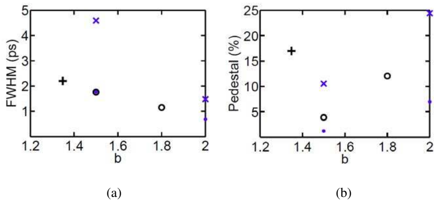
Figure 3.21: (a) FWHM (ps) and (b) pedestal (%) of the compressed pulse versus different b .
