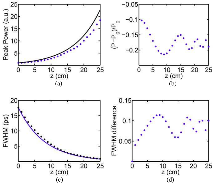
Figure 3.14: Evolution of (a) peak power (b) peak power difference (c) FWHM and (d) FWHM difference along grating length. The physical parameters are same as that of the crosses in Fig. 3.11 when b = 2.6 . The solid curve and dots represent the self-similar solution, and the results of NLCM simulation, respectively.
