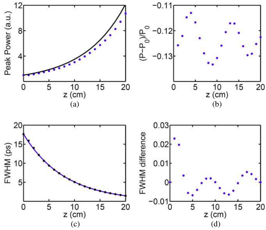
Figure 3.13: Evolution of (a) peak power (b) peak power difference (c) FWHM and (d) FWHM difference along grating length. The physical parameters are same as that of the circles in Fig. 3.11 when b = 2.2 . The solid curve and dots represent the self-similar solution, and the results of NLCM simulation, respectively.
