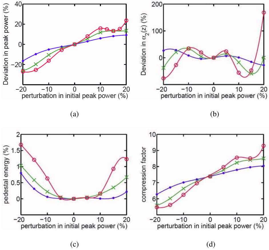
Figure 4.2: (a) Deviations of the peak power from the exact solution, (b) the chirp coefficient, (c) the pedestal energy, and (d) the compression factor at L = 400 m when the input peak power deviates from the ideal peak power from -20\% to +20\% . The physical parameters are same as those in Fig 4.1. The dots represent results for competing cubic- quintic nonlinearities ( \delta_0 = 0.4724 / \text{W}^2/\text{m} ), circles represent results for cooperating cubic- quintic nonlinearities ( \delta_0 = -0.4724 / \text{W}^2/\text{m} ), and crosses represent results for pure cubic nonlinearity ( \delta_0 = 0 ).
