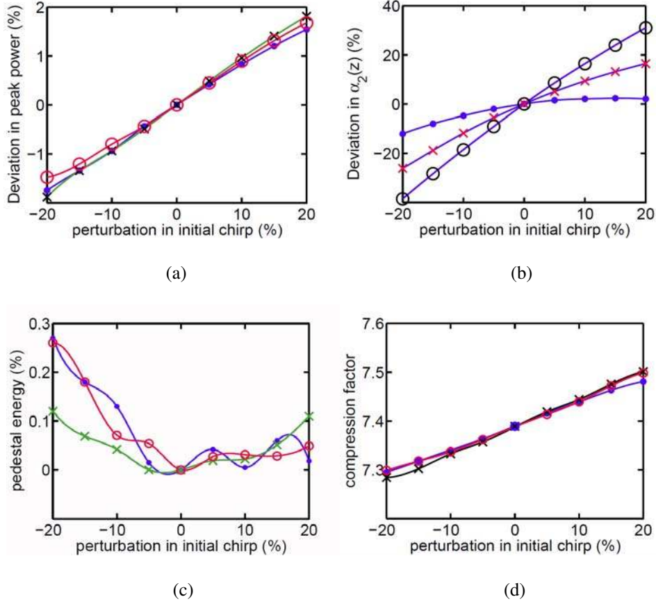
Figure 4.3: (a) Deviations of the peak power from the exact solution, (b) the chirp coefficient, (c) the pedestal energy, and (d) the compression factor at L = 400 m when the initial chirp deviates from the chirp value of the exact solution from -20\% to +20\% . The physical parameters are same as those in Fig 4.2. The dots represent results for competing cubic and quintic nonlinearities ( \delta_0 = 0.4724 /W^2/m ), circles represent results for cooperating cubic and quintic nonlinearities ( \delta_0 = -0.4724 /W^2/m ), and crosses represent results for pure cubic nonlinearity ( \delta_0 = 0 ).
