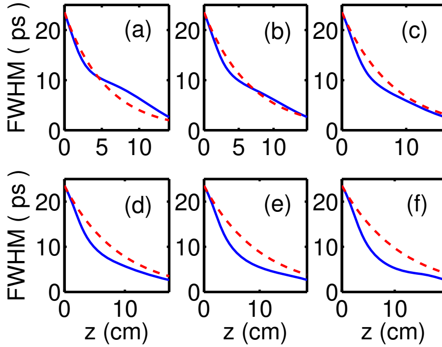
Figure 2.9: Evolution of the FWHM versus distance for different values of the ratio L_{D0,Gauss}/L_{N0,Gauss} . The dashed curve represents self-similar solitons, and the solid curve represents simulation results. The values of ratio L_{D0,Gauss}/L_{N0,Gauss} from (a) to (f) are 1, 1.2, \sqrt{2} , 1.6, 1.8 and 2, respectively.
