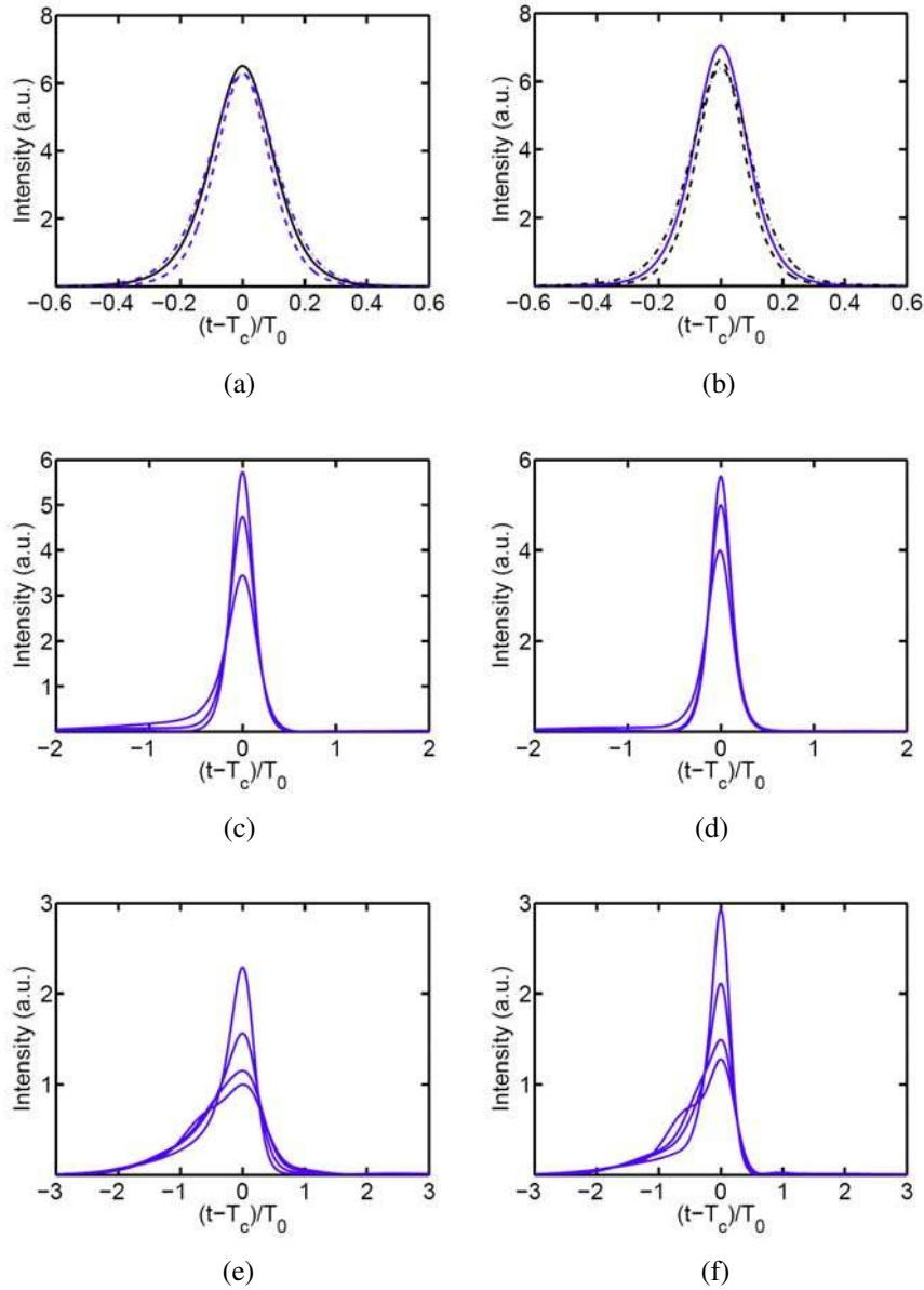
Figure 3.10: Compressed pulse when chirped hyperbolic secant pulse is the initial pulse with (a) b = 1.5 (dashed curve), b = 2 (solid curve), b = 2.5 (dot-dashed curve); (c) b = 3, 3.5, 4 (peak power from high to low); (e) b = 4.5, 5, 5.5, 6 (peak power from high to low). Compressed pulse when chirped Gaussian pulse is the initial pulse with (b) b = 1.5 (dashed curve), b = 2 (solid curve), b = 2.5 (dot-dashed curve); (d) b = 3, 3.5, 4 (peak power from high to low); (f) b = 4.5, 5, 5.5, 6 (peak power from high to low). The physical parameters are same as that in Fig. 3.9.
