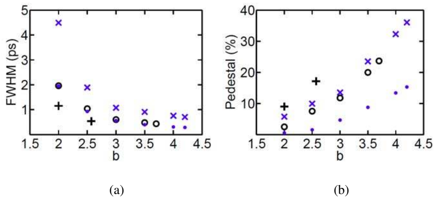
Figure 3.20: (a) FWHM (ps) and (b) pedestal (%) of the compressed pulse versus different b . Dots: \beta_{20} = -25 \text{ ps}^2/\text{cm} , T_0 = 10 \text{ ps} , \alpha_{20} = -0.005 \text{ THz}^2 ; circles: \beta_{20} = -25 \text{ ps}^2/\text{cm} , T_0 = 10 \text{ ps} , \alpha_{20} = -0.01 \text{ THz}^2 ; crosses: \beta_{20} = -25 \text{ ps}^2/\text{cm} , T_0 = 20 \text{ ps} , \alpha_{20} = -0.005 \text{ THz}^2 ; plus signs: \beta_{20} = -25 \text{ ps}^2/\text{cm} , T_0 = 5 \text{ ps} , \alpha_{20} = -0.04 \text{ THz}^2 .
