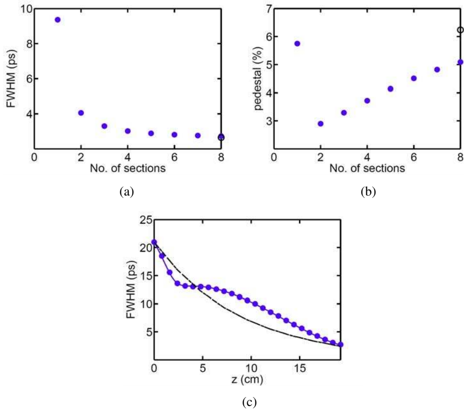
Figure 2.10: Hyperbolic secant input pulse and SWA to the exponentially decreasing dispersion. (a) The FWHM and (b) pedestal of final compressed pulse using 1 to 8 sections for SWA (dots) and DDFBG (circle). (c) Evolution of the FWHM in the DDFBG (solid curve), the 8-section SWA using the full simulation (dots), the LVM with hyperbolic secant pulse ansatz and 8-section SWA (dashed curve), and the POM with hyperbolic secant pulse ansatz and 8-section SWA (dot-dashed curve).
