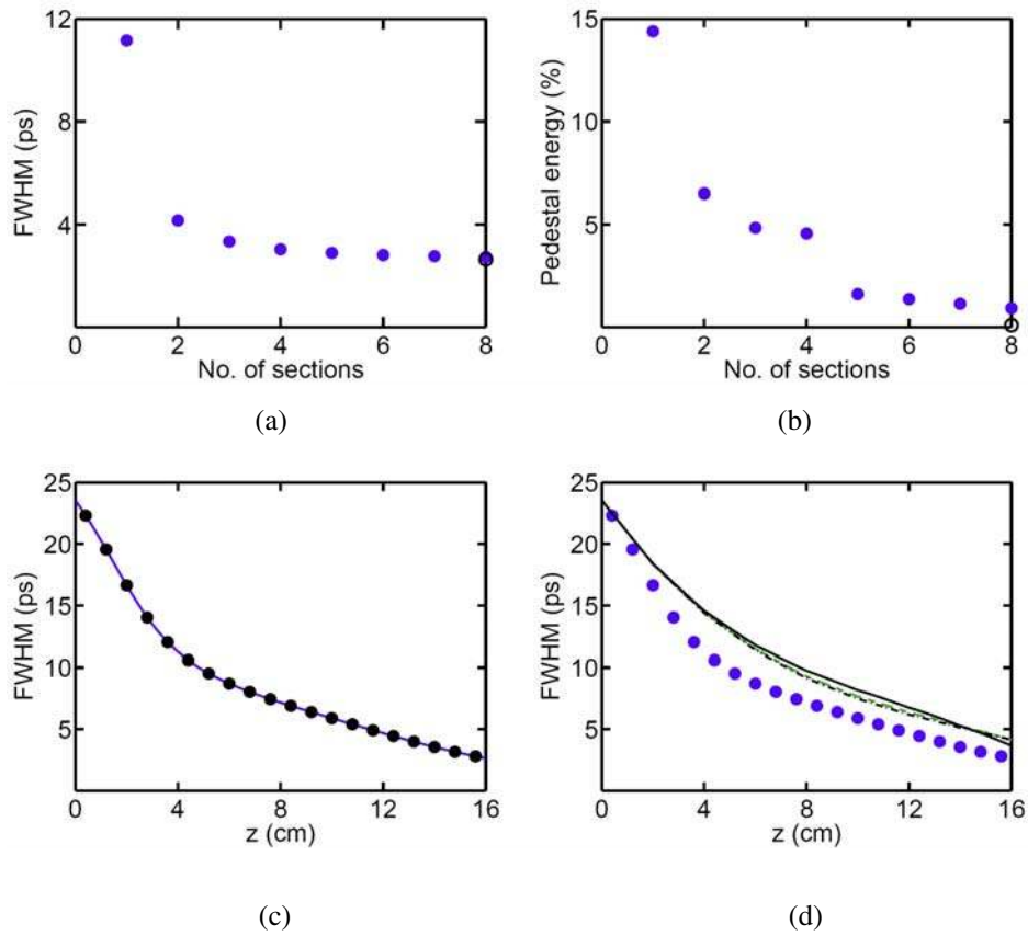
Figure 2.11: Gaussian input pulse and SWA to the exponentially decreasing dispersion. (a) Evolution of the (a) FWHM and (b) pedestal of the final compressed pulse using 1 to 8 sections for SWA (dots) and DDFBG (circle). (c) Evolution of the FWHM in DDFBG (solid curve) and 8-section SWA using full numerical simulation (dots). (d) Evolution of FWHM for the full numerical simulation on 8-section SWA (dots), the LVM with hyperbolic secant pulse ansatz and 8-section SWA (dashed curve), the POM with hyperbolic secant pulse ansatz and 8-section SWA (dot-dashed curve), and Gaussian pulse ansatz and 8-section SWA (solid curve).
