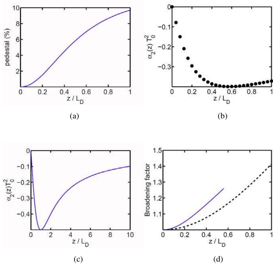
Figure 2.6: (a) Pedestal generated and (b) evolution of \alpha_2(z)T_0^2 in the chirping of a hyperbolic secant pulse using a linear FBG as a function of grating length. (c) The evolution of \alpha_2(z)T_0^2 in the chirping of a Gaussian pulse using a linear FBG versus grating length. (d) Evolution of the broadening factor until the maximum chirp occurs. The solid curve and dashed curve represent the broadening factor in the chirping of a hyperbolic secant and Gaussian pulse. The parameter L_D is the dispersion length of the linear grating.
