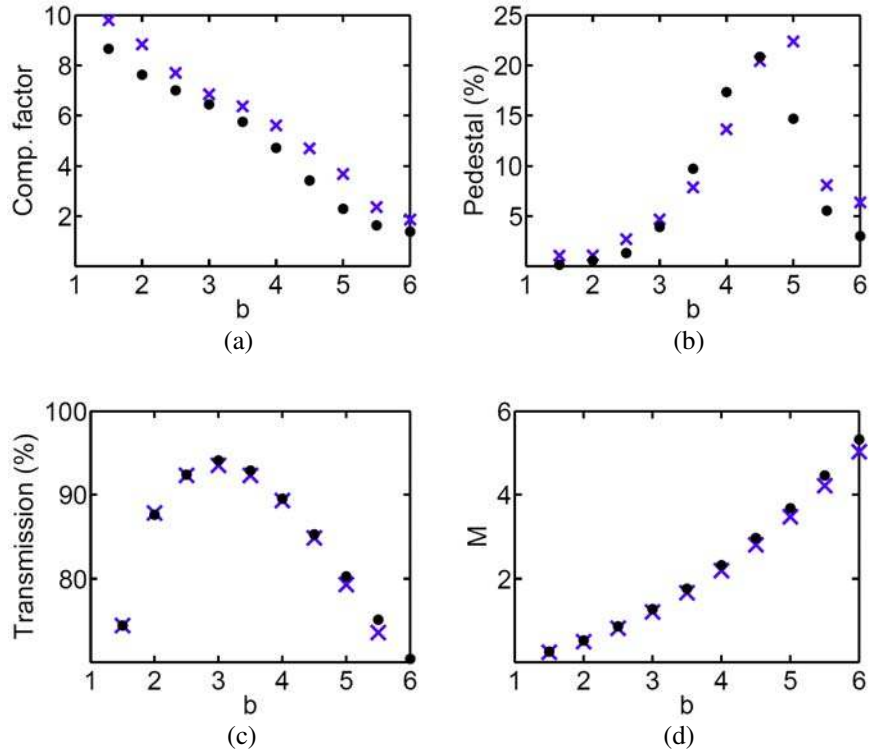
Figure 3.9: (a) Compression factor (b) pedestal (%) (c) transmission (%) (d) M versus b ( = 1.5, 2, 2.5, 3, 3.5, 4, 4.5, 5, 5.5 and 6 ). Chirped hyperbolic secant pulse (dots, \text{sech}(t/T_0) \exp(i\alpha_{20}t^2/2) , FWHM = 17.63 ps, \alpha_{20} = -0.005 \text{ THz}^2 ) and chirped Gaussian pulse (crosses, \exp(-t^2/2/T_0^2) \exp(i\alpha_{20}t^2/2) , FWHM = 17.63 ps, \alpha_{20} = -0.005 \text{ THz}^2 ) are launched into the NFBGs with exponentially decreasing dispersion. The grating parameters are \beta_{20} = -25 \text{ ps}^2/\text{cm} , \sigma = 0.125 \text{ /cm} , \gamma = 5 \text{ /W/km} and L = 16 \text{ cm} .
