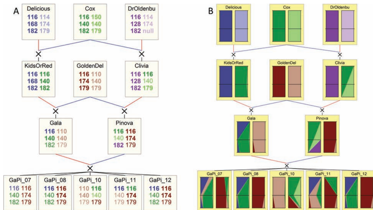
Figure 5. The same apple pedigree as in the first 3 figures is shown with precalculated IBD data for part of chromosome 1. Panel A shows the most probable founder alleles instead of the observed alleles. The color of the allele indicates the founder allele. A bold typeface indicates a high probability, normal and italic typefaces indicate lower probabilities according to user-specified thresholds. In panel B, again each color represents a different founder haplotype. Each rectangle in an individual represents 1 of the 2 copies of the selected chromosome. The vertical dimension represents the positions along the chromosome; the width of a color at a certain position indicates the IBD probability that the corresponding founder allele is present.
