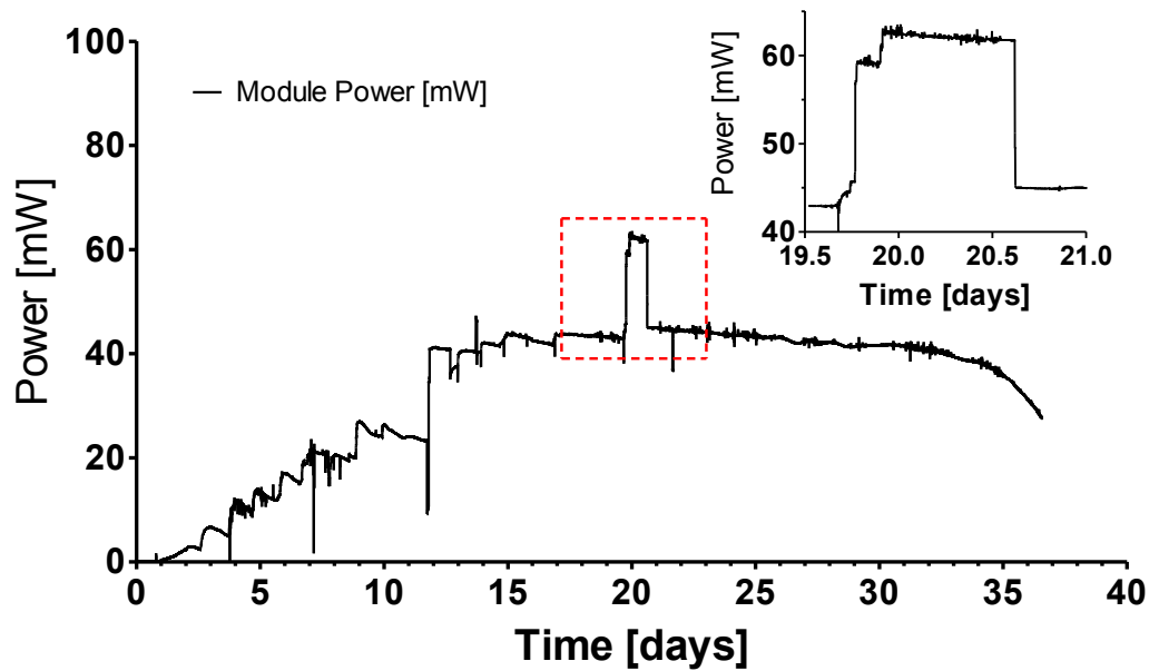
Figure 3. Real time power output from a single module of 36 MFCs connected in parallel. Inset graph is a magnification of the marked area, where the load was changed to 2.3\Omega for approximately 24 hours.
