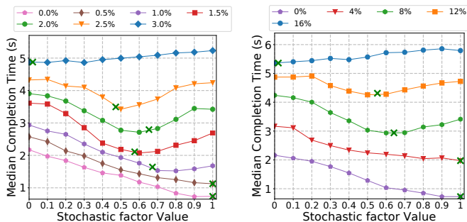
(a) LinUCB with loss
