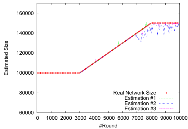
Figure 14: Aggregation : Growing network, 100,000 node network
