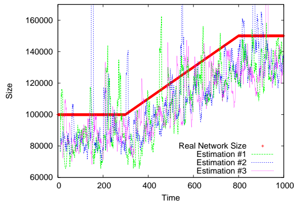
Figure 11: HopsSampling : Last10runs heuristic, 100,000 node network, growing network
