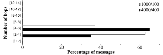
Fig. 3. Distributions of unicast message hops. Average group size is 10. No message aggregation.
