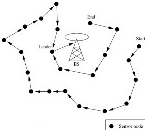
Figure 2: Illustration of PEGASIS protocol
