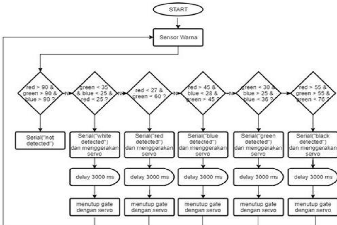
Gambar 4. Flowchart Sistem
