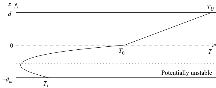
FIGURE 3. Steady-state temperature profile, case 2: depth z against temperature T .
