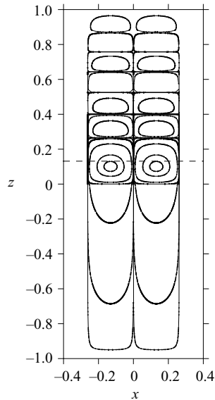
FIGURE 8. Streamline plot from the Q model, type 4, T_U = 9^\circ\text{C} , \hat{d} = 1 , \delta = 0.002 , \hat{\epsilon} = -0.025 , \hat{\epsilon}_m = -0.0728 , Ra_m = 8.839 , a_m = 12 .
