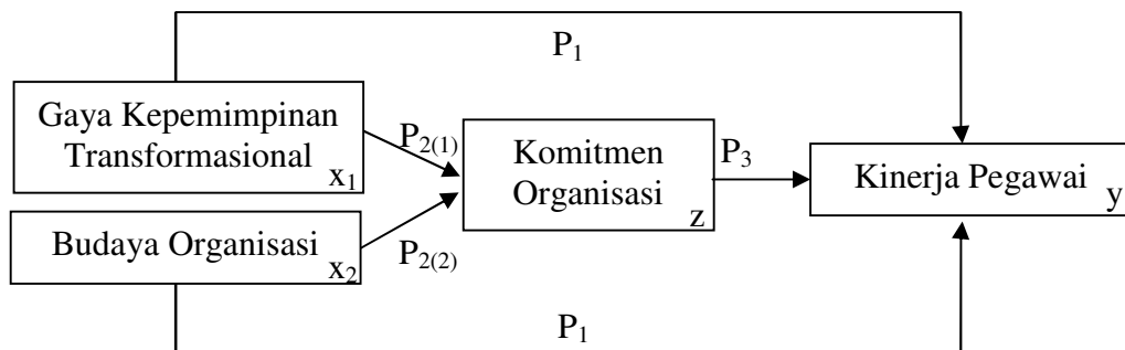
Gambar 2 Path Analysis
