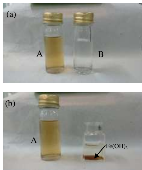
Figure 1. Physical properties of 100 mg Fe/L (a) at feed pH 9.3 (sample A), pH 6.5 (sample B) and (b) when Fe(OH)_3 formed as flocs
