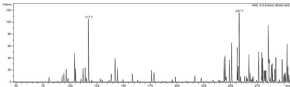
Figure 4. Valine MS-spectra
