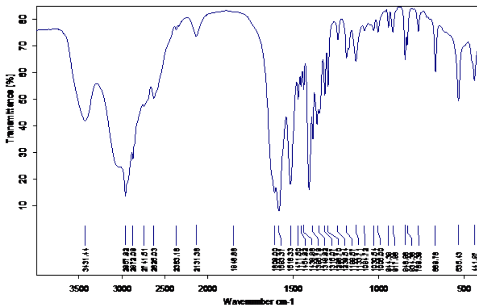
Figure 2. FT-IR spectra of leucine
