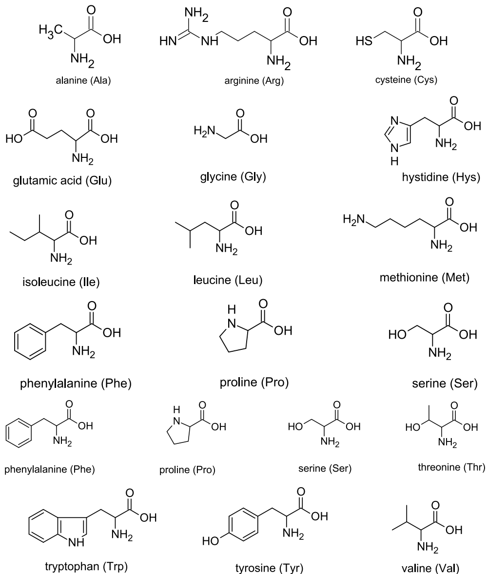
Figure 1. Amino acids chemical structures
