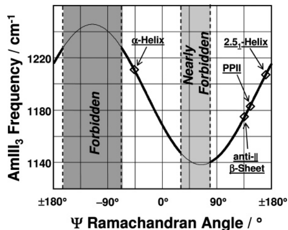
Figure 5. Refinement of correlation between AmIII 3 frequency and \Psi Ramachandran angle for non-HB PB, which reflects only coupling between N–H and C \alpha –H bending motions, as predicted earlier for AMA. 47 (A) ( \diamond ) AmIII 3 frequencies where the HB-induced frequency upshifts were subtracted from the experimentally measured values (see Appendix). (B) Black curve shows the best fit of these data (eq 5). Note: Gray regions show the sterically forbidden/nearly forbidden \Psi Ramachandran angles based on recent Ramachandran plots for non-Gly, non-Pro, and nonpre-Pro residues. 90–92
