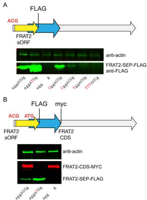
Fig. 5. Characterization of the non-AUG initiation codon of the FRAT2-SEP sORF (a) An ACG was confirmed as the FRAT2-SEP initiation codon by site-directed mutagenesis followed by western blots of FRAT2-SEP-FLAG using an anti-FLAG antibody. Conversion of the ACG to an ATG resulted in higher expression (lane 2), while ablation of this codon removed all expression (lane 3). In addition, perturbation of the Kozak sequence (lanes 4-7) revealed the importance of context when using non-AUG codons, as substitution of less favorable residues 29 at the most important positions in the Kozak sequence resulted in lower FRAT2-SEP-FLAG expression. (b) Epitope tagging of the sORF and CDS of the FRAT2 mRNA demonstrates that the FRAT2 mRNA is bi-cistronic. Specifically, the FRAT2 CDS was c-myc tagged and the FRAT2-SEP was FLAG tagged. Conversion of the FRAT2-SEP initiation codon from ACG to ATG ablates the expression of the downstream FRAT2-CDS , indicating the importance of alternate start codons for polycistronic expression. (Note: RNA maps are not to scale. See Supplementary Fig. 12 for lengths of the RNAs and sORFs.)
