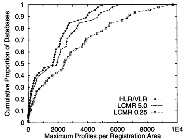
Figure 11. Cumulative distribution of maximum required storage for profiles.
