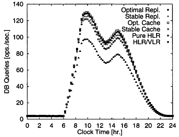
Figure 7. System-wide database lookups.
