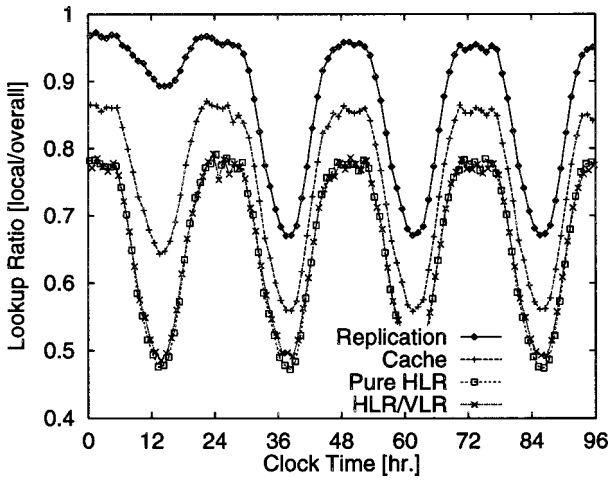
Figure 5. Percentage of calls serviced by local lookups [4-days simulation].
