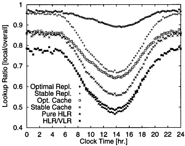
Figure 6. Percentage of calls serviced by local lookups [1-day simulation].
