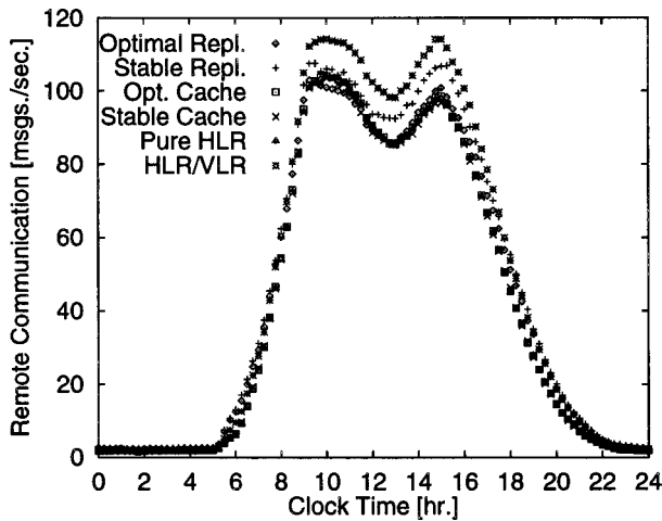
Figure 9. Average number of network messages.
