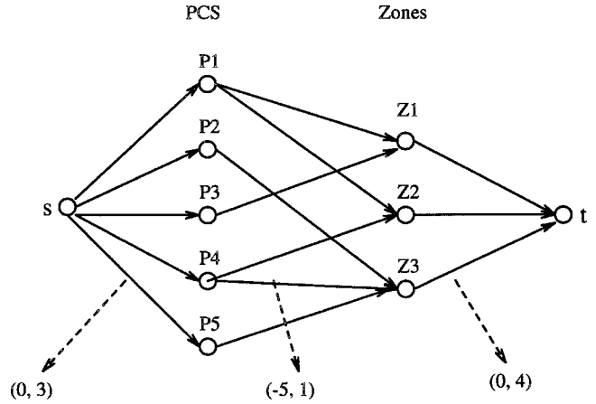
Figure 2. Example of a flow network.
