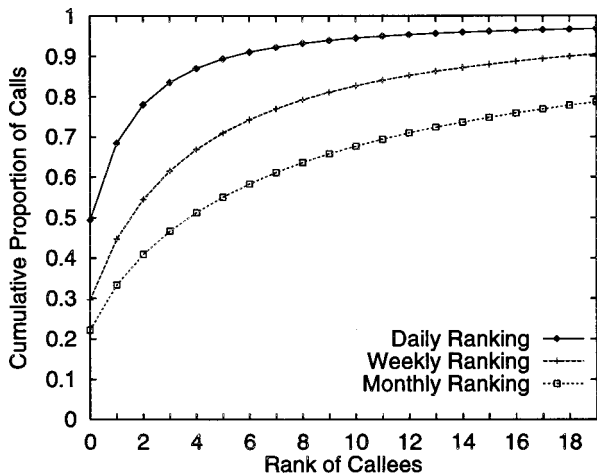
Figure 1. Locality in calling patterns.
