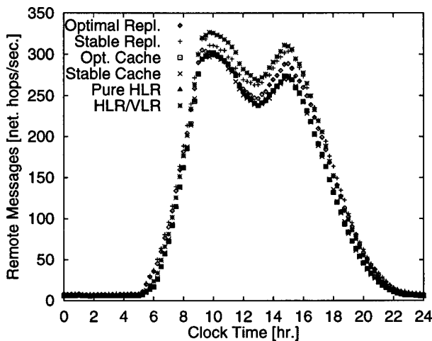
Figure 10. Average number of network message hops.
