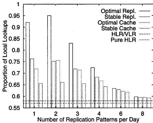
Figure 12. Change in performance with number of reallocations per day.
