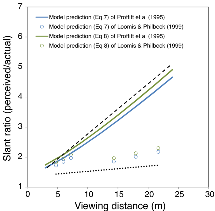
Figure 10. Modeled proportional slant overestimation as a function of viewing distance from the aspect-ratio data in Experiment 2 . The green (VHI-corrected) and blue (uncorrected) curves are the model predictions for the viewing conditions of Proffitt et al. (1995; Experiment 1 ). The circles are the corresponding model predictions for the viewing conditions of Loomis and Philbeck (1999; binocular condition with physical ratio of 1.5). Dashed lines represent linear trend lines from the corresponding empirical data (see Figure 2 ).
