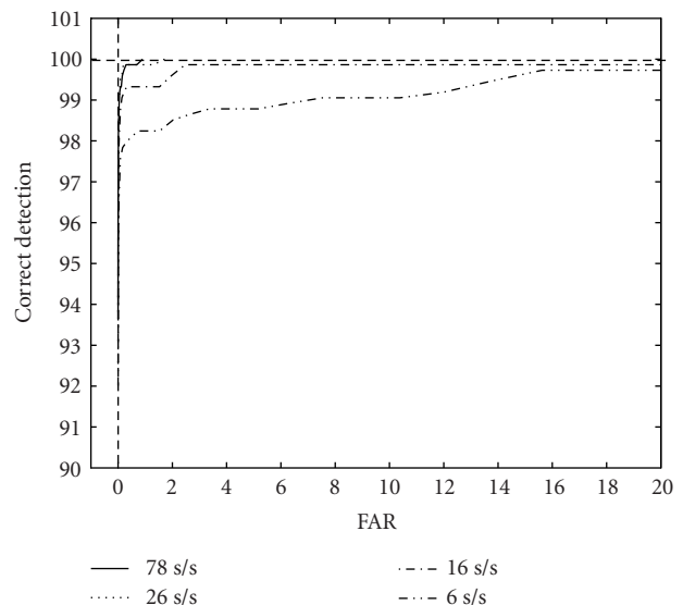
FIGURE 10: Receiver operating characteristics for different hash sizes in samples/s (s/s). 78 s/s: 3 SVDs, 25-millisecond frame length; 26 s/s: 1 SVD, 25-millisecond frame length; 16 s/s: 1 SVD, 40-millisecond; 6 s/s: 1 SVD, 100-millisecond frame length.
