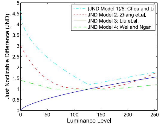
Fig. 3. Luminance Masking/Adaptation (Just Noticeable Difference) Models.
