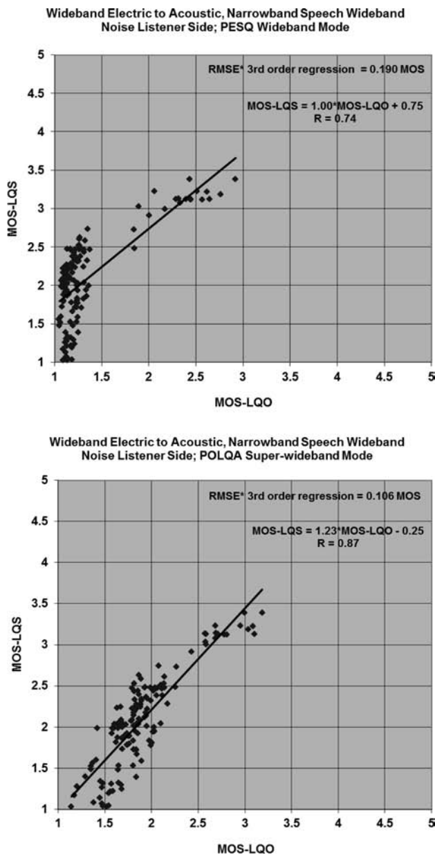
Fig. 12. Comparison of PESQ and POLQA results for the wideband electric to acoustic database with narrowband speech and wideband background noise. The average root mean square error, corrected for the 95% confidence interval (RMSE*), using a 3 rd order regression between subjective and objective results, drops from 0.19 down to 0.11 MOS, while the linear correlation increases from 0.74 to 0.87.
