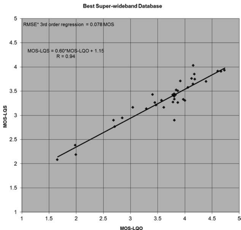
Fig. 10. POLQA result for the best case super-wideband experiment using all phase 1 and phase 2 subjective tests. The average root mean square error, corrected for the 95% confidence interval (RMSE*), using a 3 rd order regression between subjective and objective results, is 0.08 MOS. The linear correlation is excellent (0.94), the significant deviation from ideal regression Y = X is caused by an imbalance in the subjective test that did not contain enough severe degradations with low subjective MOS scores.
