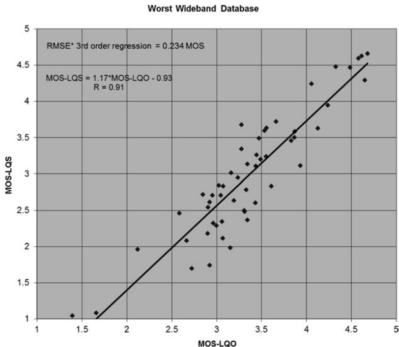
Fig. 9. POLQA result for the worst case wideband experiment using all phase 1 and phase 2 subjective tests. The average root mean square error, corrected for the 95% confidence interval (RMSE*), using a 3 rd order regression between subjective and objective results, is 0.23 MOS. The linear correlation is excellent (0.91) and close to the ideal regression Y = X .
