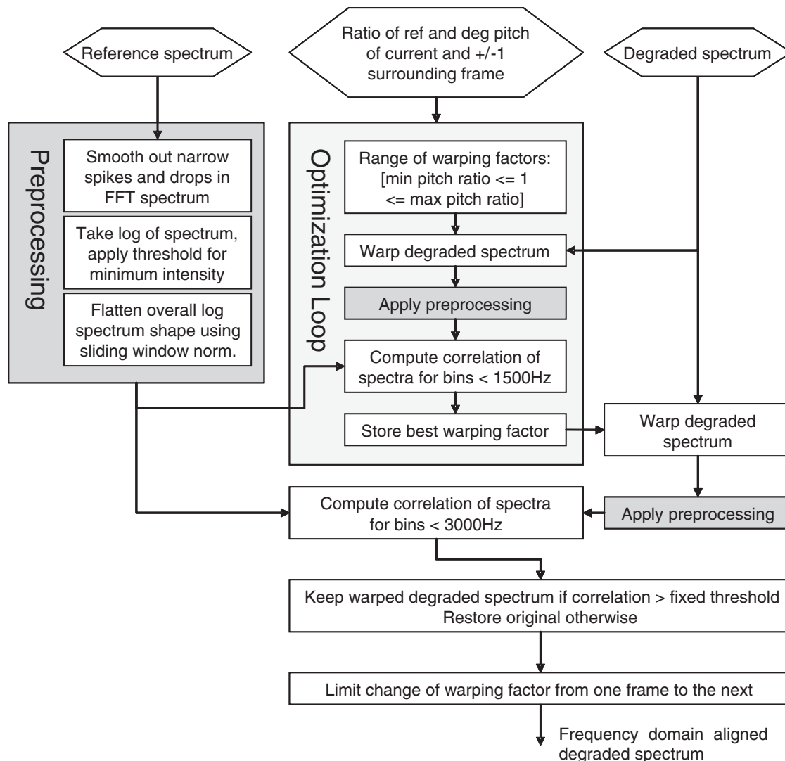
Fig. 2. Overview of the frequency domain alignment used in the POLQA perceptual model.
