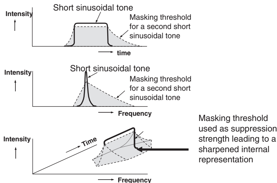
Fig. 5. Masking approach used in the POLQA perceptual model. The tent-like figure in the time-frequency plane is used to suppress the loudness of components of the signal.
