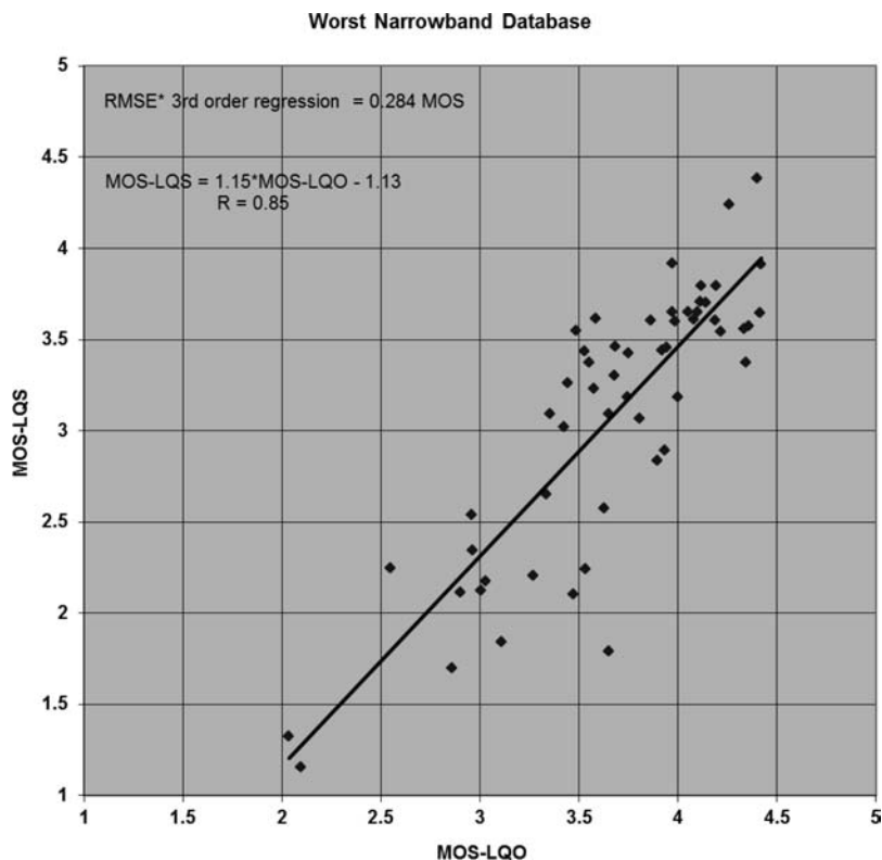
Fig. 7. POLQA result for the worst case narrowband experiment using all phase 1 and phase 2 subjective tests. The average root mean square error, corrected for the 95% confidence interval (RMSE*), using a 3 rd order regression between subjective and objective results, is 0.28 MOS. The linear correlation is very good (0.85) and close to the ideal regression Y = X .
