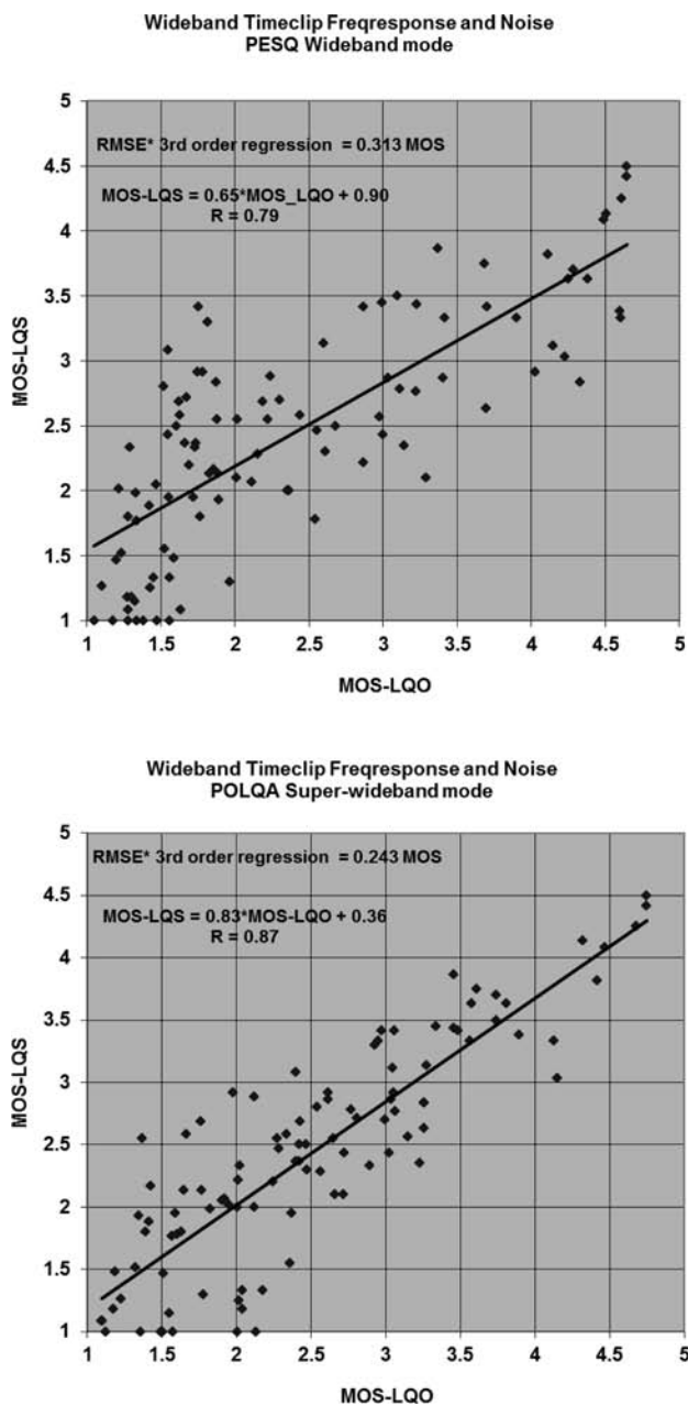
Fig. 14. Comparison of PESQ and POLQA results for the artificially generated time clipping, frequency response distortion, and background noise. The average root mean square error, corrected for the 95% confidence interval (RMSE*), using a 3 rd order regression between subjective and objective results drops from 0.31 down to 0.24 MOS for PESQ and POLQA respectively, while the linear correlation increases from 0.79 to 0.87.
