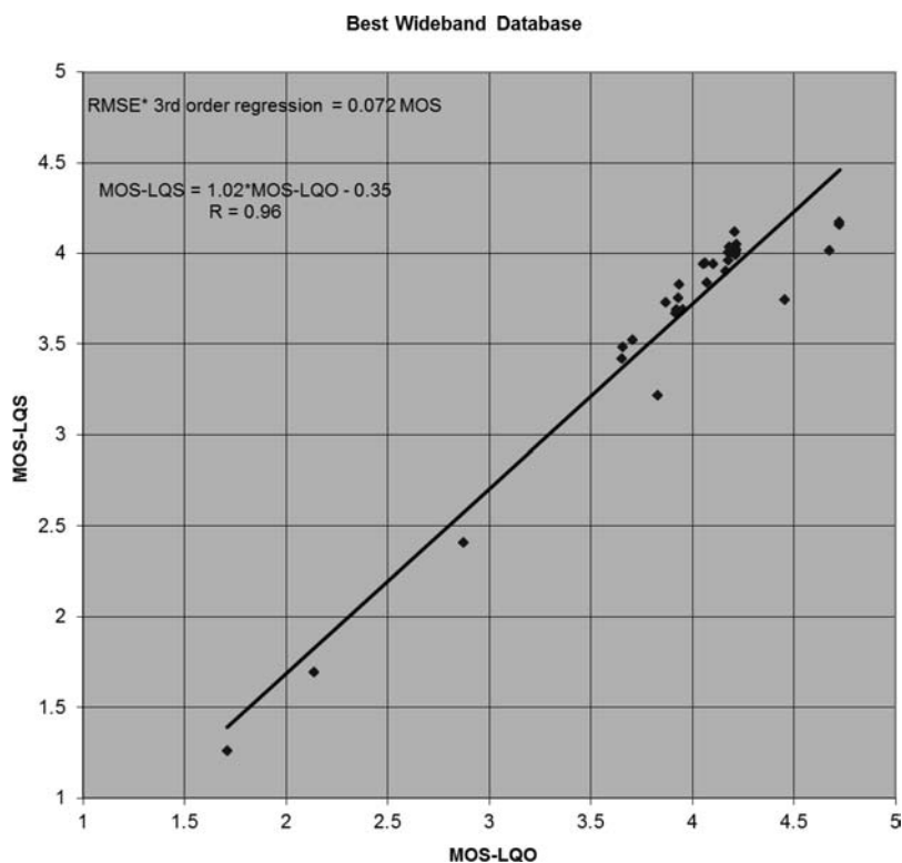
Fig. 8. POLQA result for the best case wideband experiment using all phase 1 and phase 2 subjective tests. The average root mean square error, corrected for the 95% confidence interval (RMSE*), using a 3 rd order regression between subjective and objective results, is 0.07 MOS. The linear correlation is excellent (0.96) and very close to the ideal regression Y = X .
