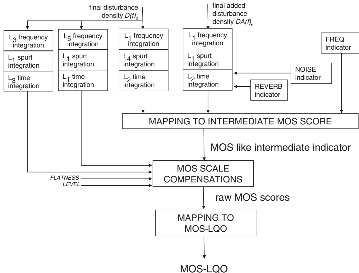
Fig. 4. Overview of the third part of the POLQA perceptual model. Calculation of the final objective listening quality MOS score (MOS-LQO) from the final disturbance densities (see Sections 2.13 and 2.14).
