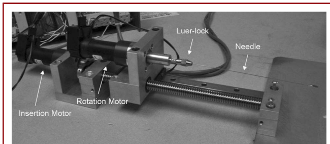
FIGURE 2. The needle-steering system developed for use in the cadaver trials.
