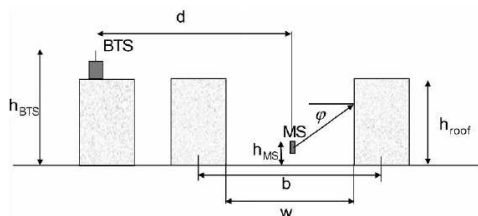
Gambar 5. Model Walfish-Ikegami.
