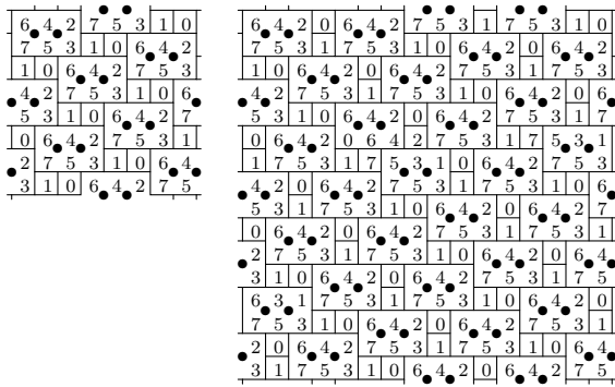
Figure 5: First two odd-weight cases: M(1) and M(01)
