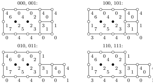
Figure 3: Labeled room-label pairs for middle entries of binary triples
