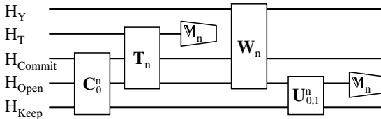
Fig. 2. The inverter \mathbf{I}_n^{\tilde{A}}(y), y \in \{0, 1\}^n obtained from adversary \tilde{A} = (C_n^0, U_{0,1}^n) .
