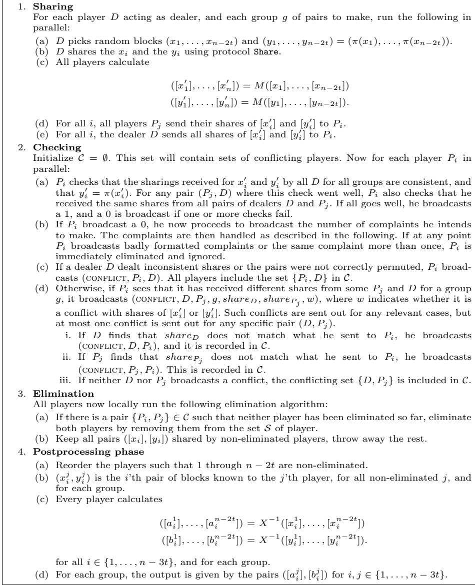
Fig. 4: Protocol RandomPairs
