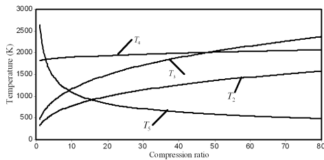
Fig. 2. The temperature versus compression ratio for \alpha = 1.5 .
