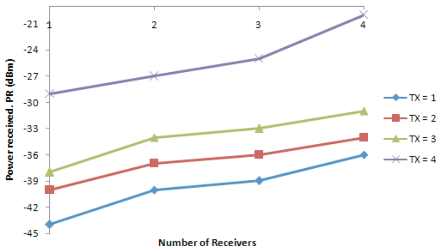
Fig. 7 Experimental received power for link range = 1 km.
