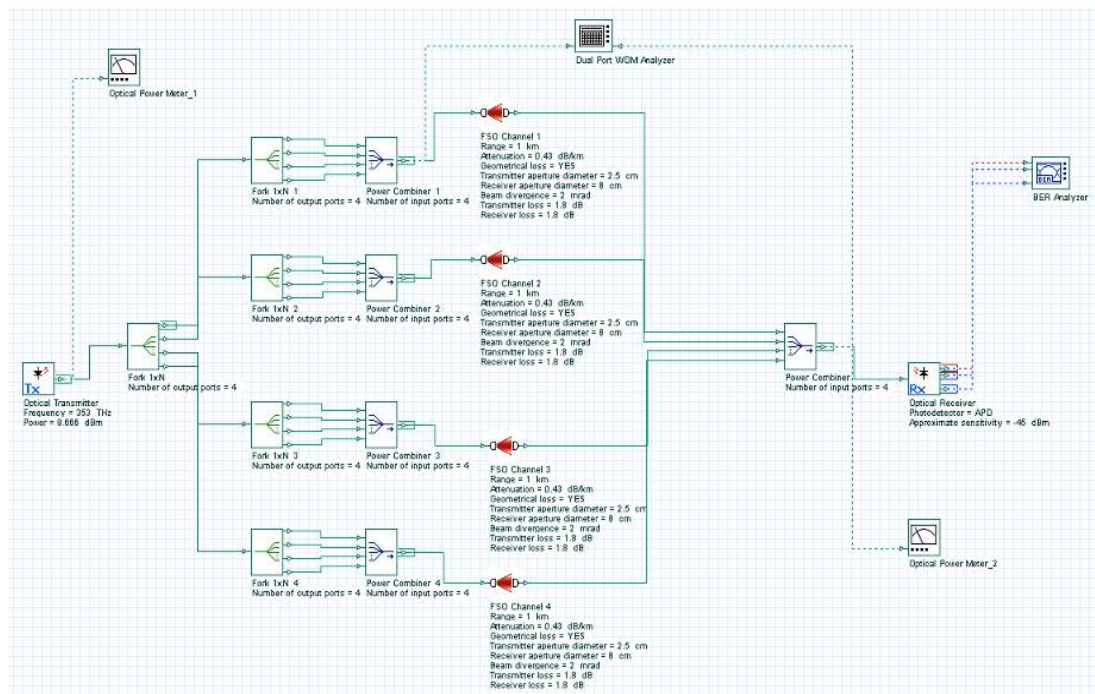
Fig. 2 TX/RX FSO link simulation layout.
