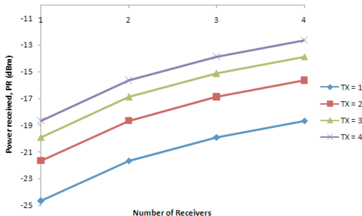
Fig. 4 Theoretical received power of doubling the number of TX and RX.
