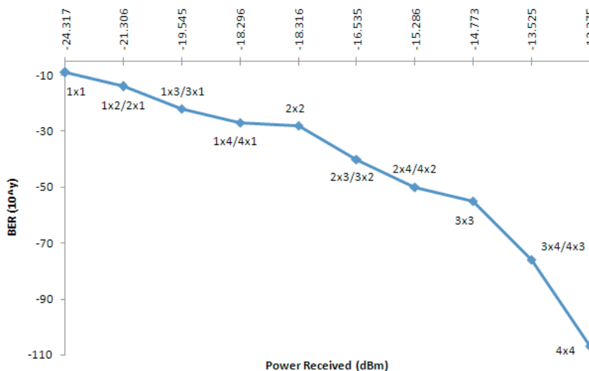
Fig. 6 BER versus power received for multiple laser beams.
