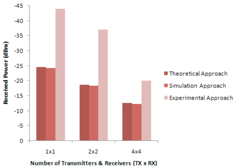
Fig. 8 Received power for doubling the number of TX and RX using theoretical, simulation and experimental approach.
