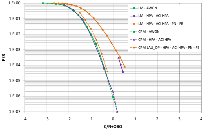
Fig. 5. PER comparison: LM vs. CPM, RCS2 waveform ID = 3, considering phase noise (PN), frequency errors (FE), and ACI
