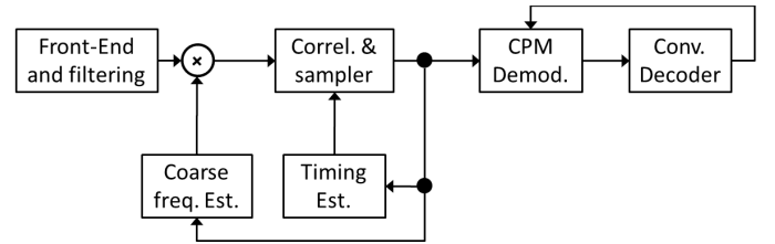
Fig. 4. Block Diagram of the CPM receiver
