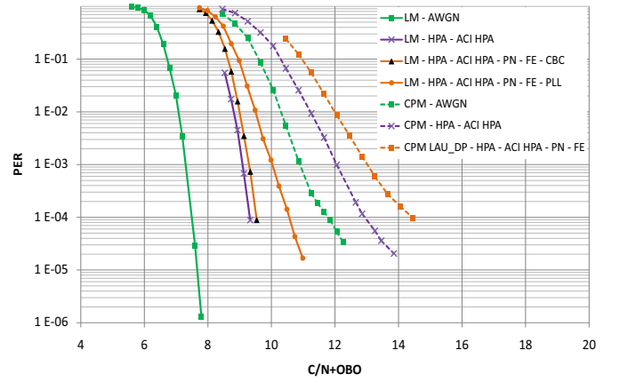
Fig. 6. PER comparison: LM vs. CPM, RCS2 waveform ID = 8, considering phase noise (PN), frequency errors (FE), and ACI
