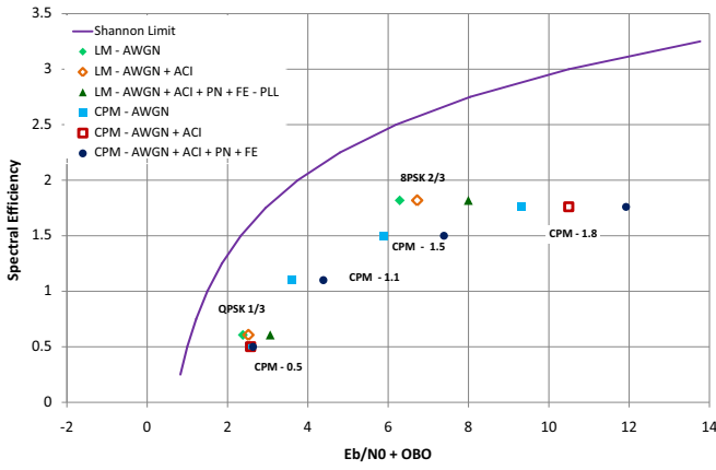
Fig. 8. Spectral Efficiency: CPM vs. LM comparison
