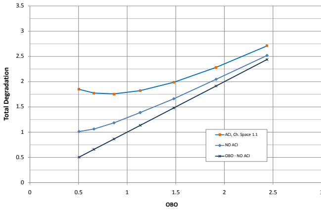
Fig. 2. Total Degradation analysis for LM waveform 8: 8PSK 2/3
