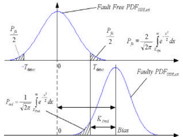
Figure 8: Minimum Detectable Bias
