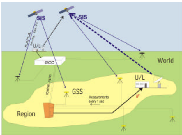
Figure 13: SISE estimation for one Galileo satellite
