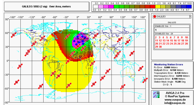
Figure 14: SISE with 8 GSS within ECAC (Snapshot)
