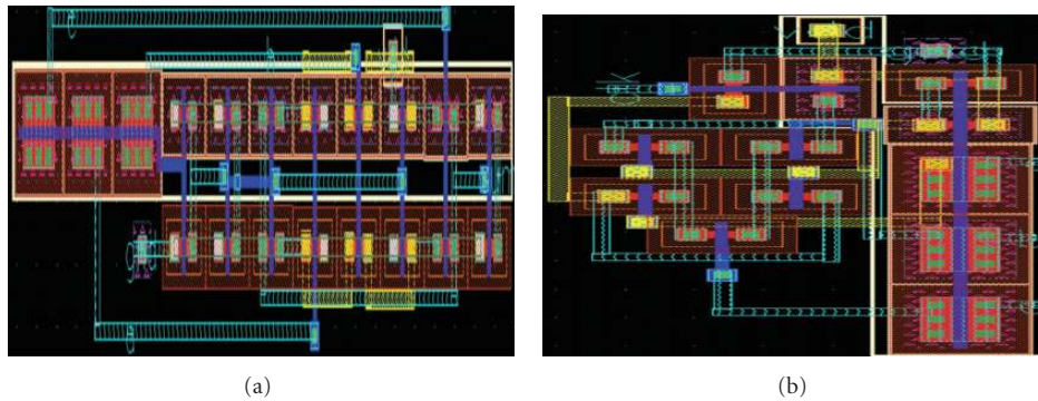
FIGURE 28: (a) Layout of design 1 (PMajFA1) full adder cell. (b) Layout of design 2 (PMajFA2) full adder cell.
