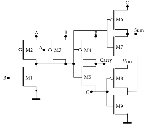
FIGURE 8: 9T full adder.
