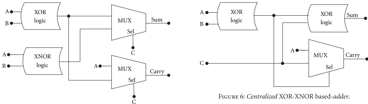
FIGURE 5: Cascaded XOR-XNOR based-adder.
