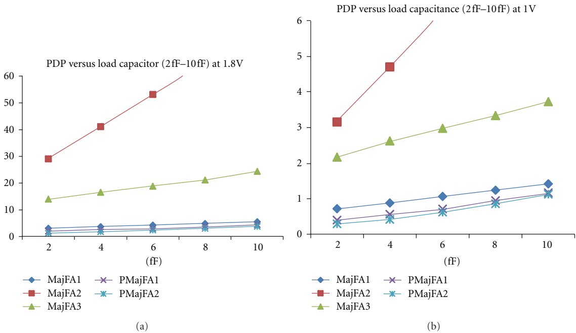
FIGURE 26: (a) PDP comparison of Majority-function-based full adder cells with capacitance load variation at 1.8 V. (b) PDP comparison of Majority-function-based full adder cells with capacitance load variation at 1 V.
