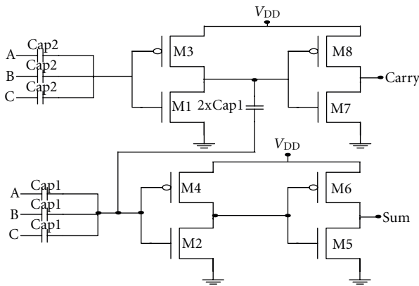
FIGURE 15: 3-input MOSCAP Majority full adder (MajFA4).
