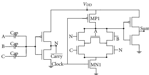
FIGURE 21: Majority function-based adder design 2 (PMajFA2).
