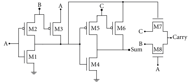
FIGURE 9: 8T full adder.
