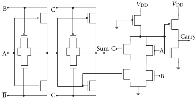
FIGURE 2: TG-Pseudo adder cell.
