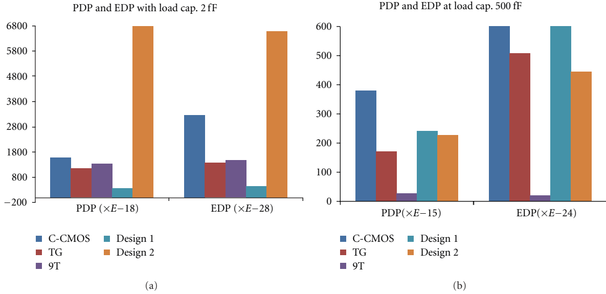
FIGURE 25: (a) PDP and EDP of XOR-XNOR based full adder cells with load capacitance (2 fF) at 1.8 V. (b) PDP and EDP of XOR-XNOR based full adder cells with load capacitance (500 fF) at 1.8 V.
