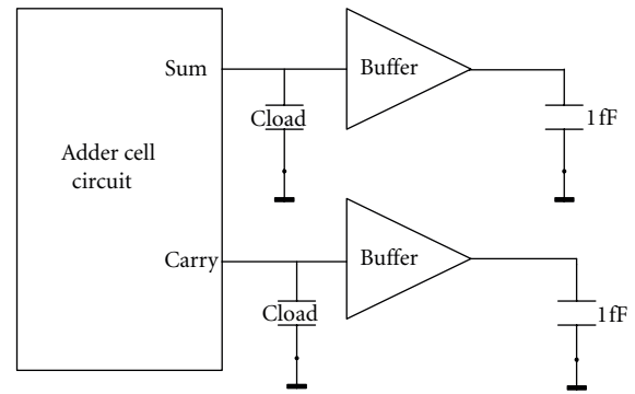
FIGURE 22: Simulation test bench for load Analysis.
