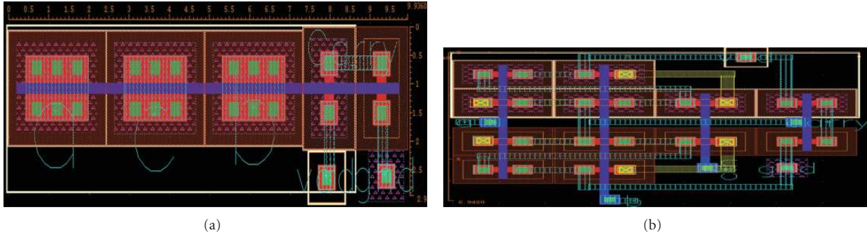
FIGURE 12: (a) MOSCAP Majority Not function layout. (b) Static CMOS bridge (Majority function) layout.
