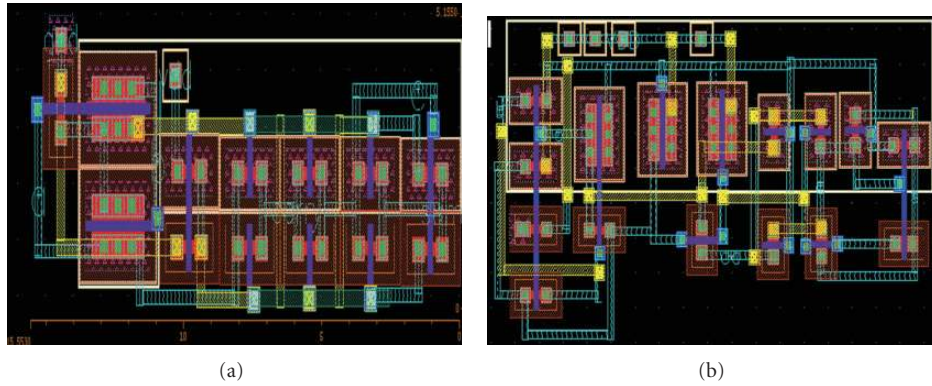
FIGURE 27: (a) Layout of design 1 (13T) full adder cell. (b) Layout of design 2 (16T) full adder cell.
