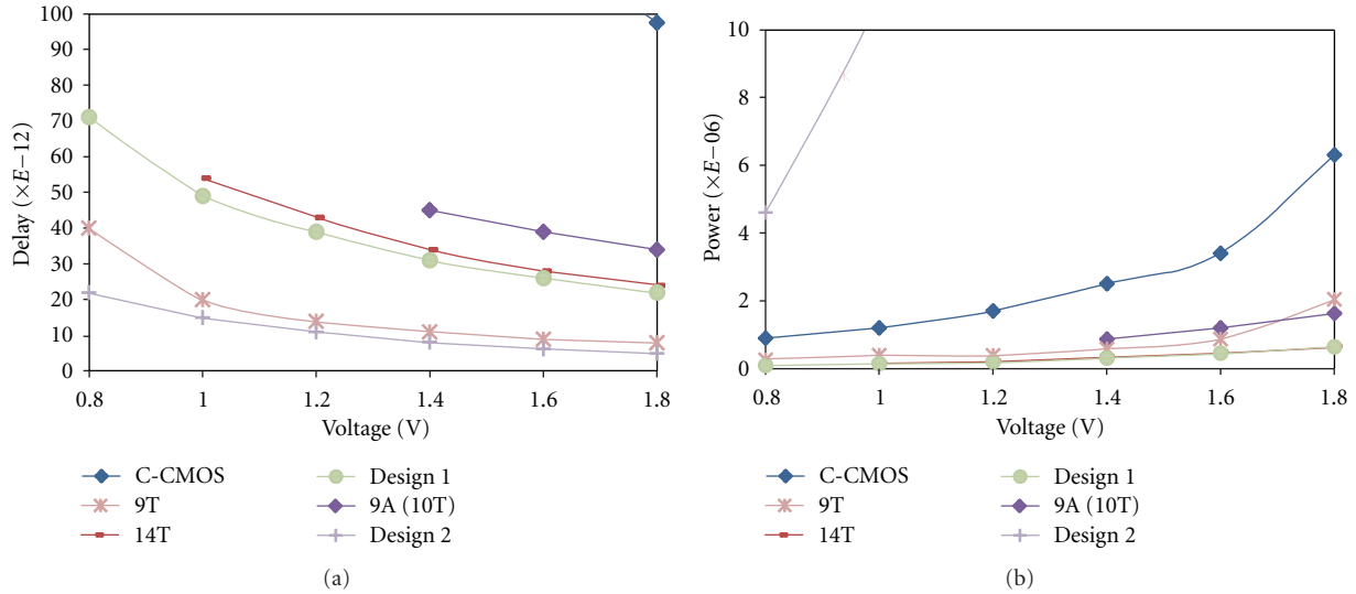
FIGURE 23: (a) Delay (ps) of XOR-XNOR-based adders. (b) Power (μW) XOR-XNOR-based adders.
