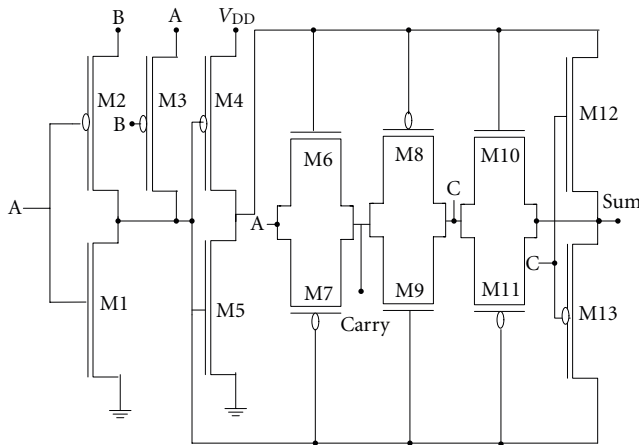
FIGURE 18: XOR- (3T-) based design 1 full adder.
