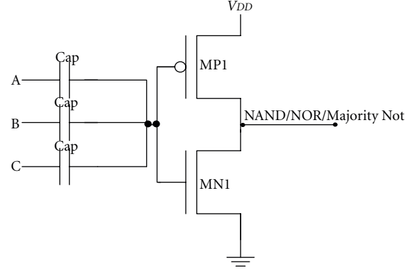
FIGURE 11: Majority function- (MOSCAP-) based logic gates.
