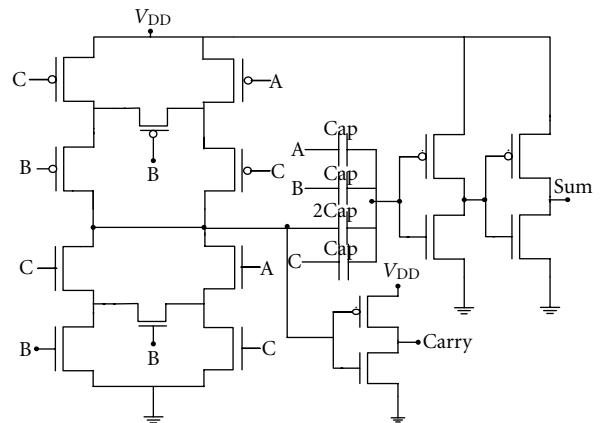
FIGURE 16: 5-input MOSCAP Majority full adder (MajFA5).
