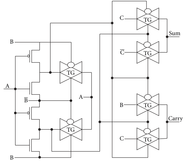
FIGURE 3: TG adder cell.
