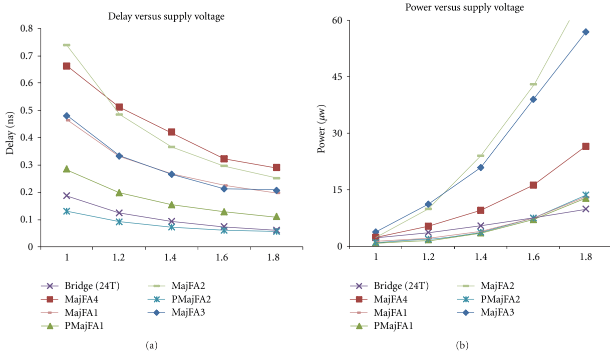
FIGURE 24: (a) Delay of Majority-function-based full adder circuits. (b) Power of Majority-function-based full adder circuits.
