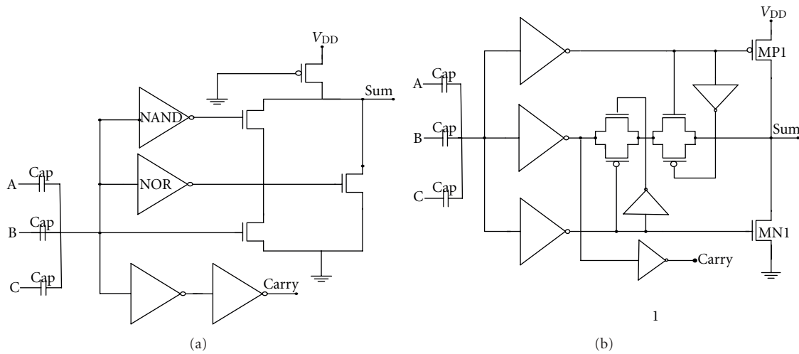
FIGURE 14: (a) Majority-function-based full adder (MajFA2). (b) Inverter-based Majority full adder (MajFA3).
