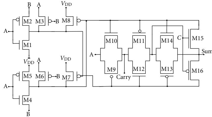
FIGURE 19: XOR-XNOR- (3T-) based design 2 full adder.
