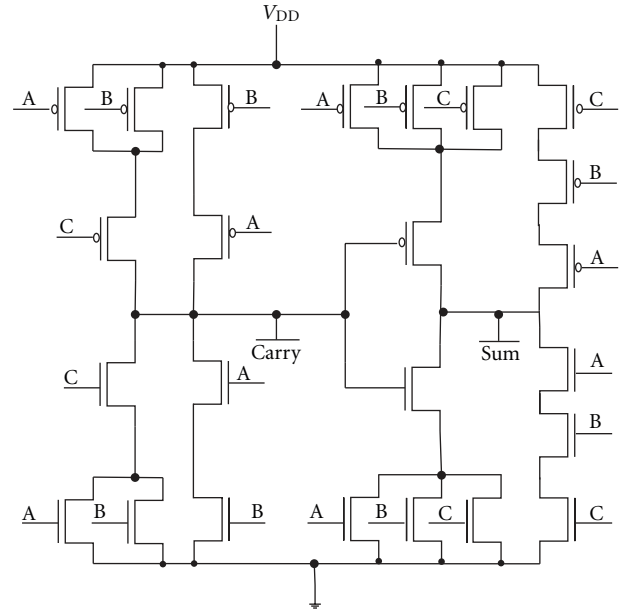
FIGURE 1: C-CMOS adder cell.
