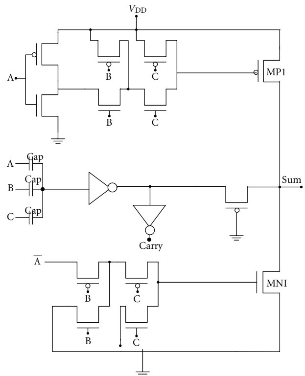
FIGURE 13: Design methodologies for Majority-function-based full adder (MajFA1).
