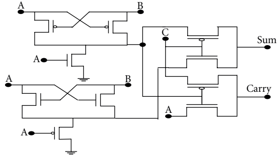
FIGURE 7: XOR-XNOR- (3T-) based 10T full adder.
