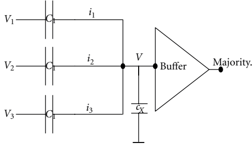
FIGURE 10: Implementation of Majority functions (MOSCAP).
