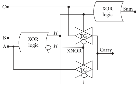
FIGURE 17: General structure of proposed XOR-XNOR-based adder.
