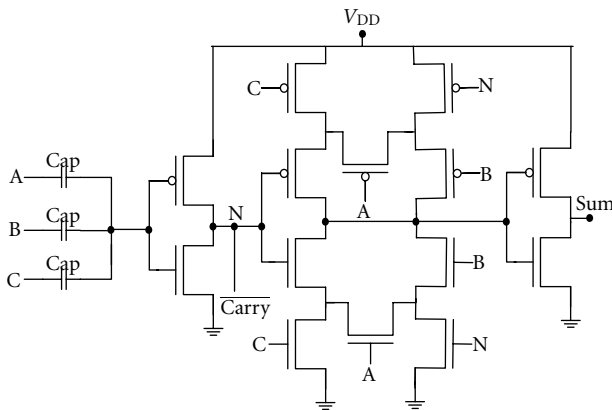
FIGURE 20: Majority-function-based adder design 1 (PMajFA1).
