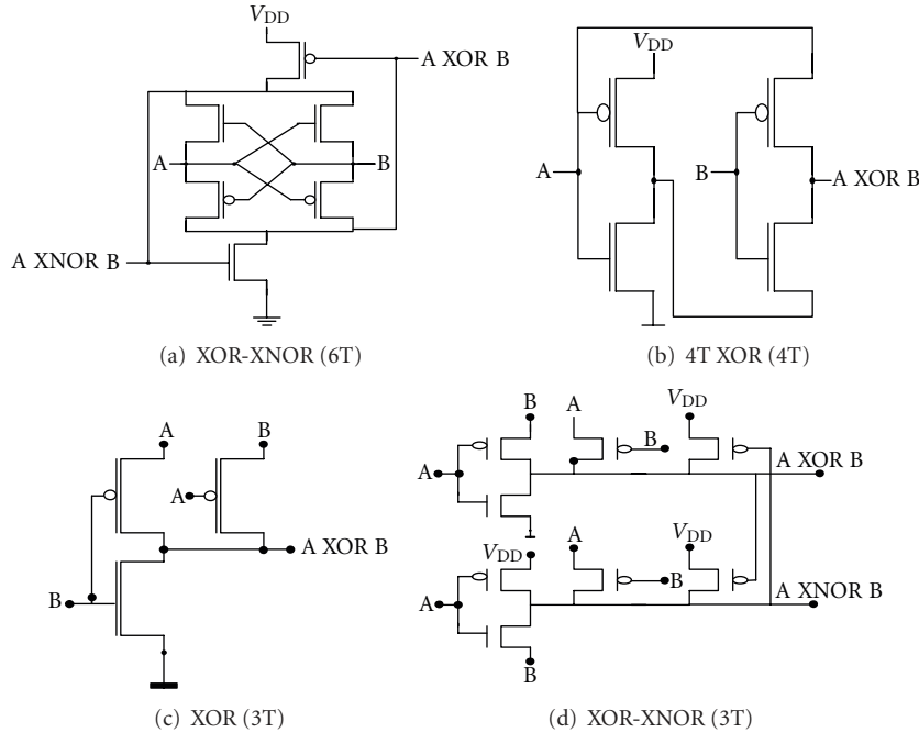
FIGURE 4: Basic designs of XOR-XNOR gate found in literature.
