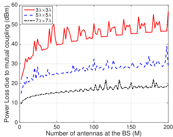
Fig. 9: Power loss due to mutual coupling with respect to M considering different array dimensions.
