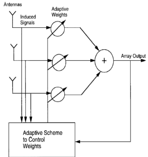
Fig.1. Smart/adaptive antenna array system
