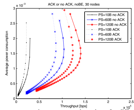
Fig. 9. Power consumption versus net throughput for different packet sizes in case of acknowledged and unacknowledged traffic.
