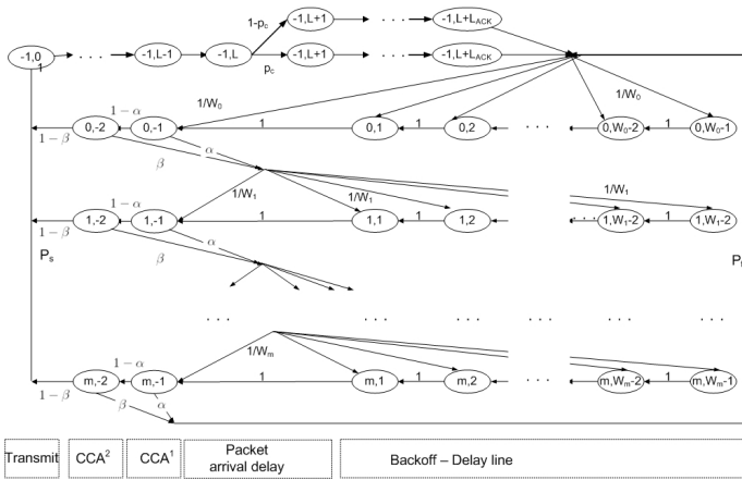
Fig. 3. Markov Model for IEEE 802.15.4
