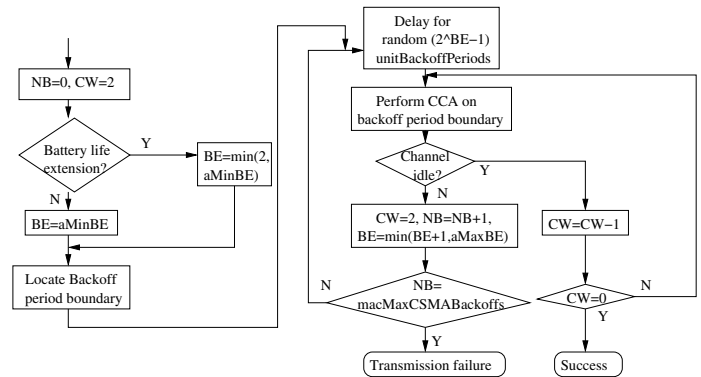
Fig. 2. Backoff mechanism for 802.15.4 CSMA
