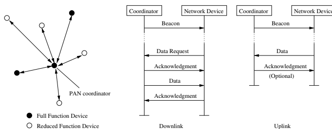
Fig. 1. Transmission schemes in a one-hop star 802.15.4 network. In the case of uplink transmission (monitoring scenario), the use of the acknowledgement is optional. In this paper, we model the network with and without acknowledgement to be able to address the performance of both possibilities.
