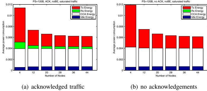
Fig. 8. Energy cost breakdown: Tx energy - Rx energy - CCA energy - Idle energy
