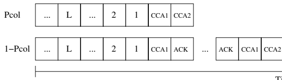
Fig. 4. Slot timing for the derivation of \beta , in case of an acknowledged transmission.
