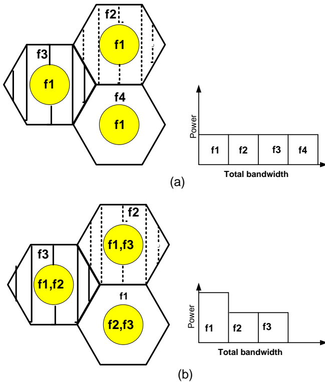
Fig. 1. FFR Concept. a) Strict FF. b) SFR.
