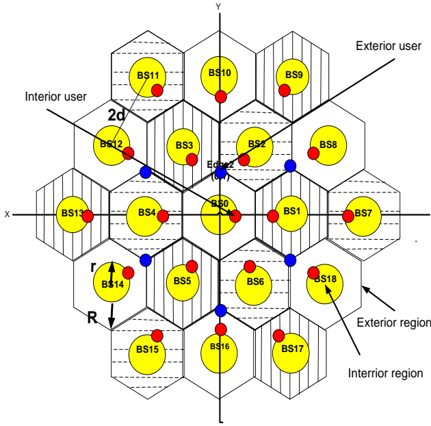
Fig. 2. Two-tier network with FFR three
