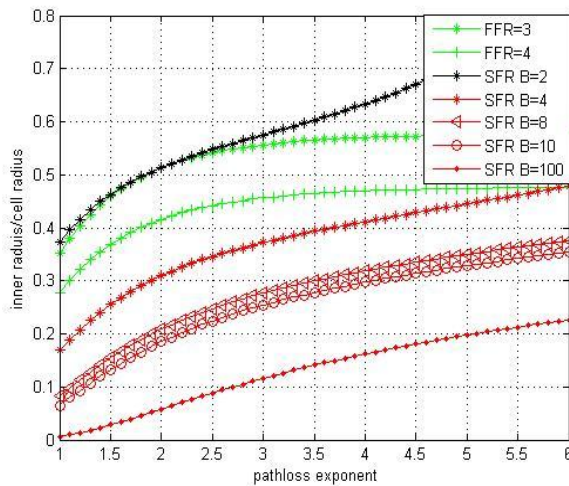
Fig. 6. Inner radius to cell radius ratio vs. path loss exponent at no power control ( \mu=0 )
