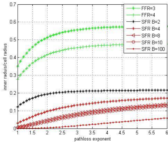
Fig. 7. Inner radius to cell radius ratio vs. path loss exponent at power control ( \mu=0.6 )
