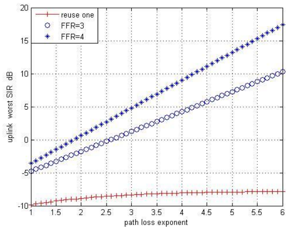
Fig. 4. worst SIR vs. path loss exponent for reuse1, FFR3, and FFR4
