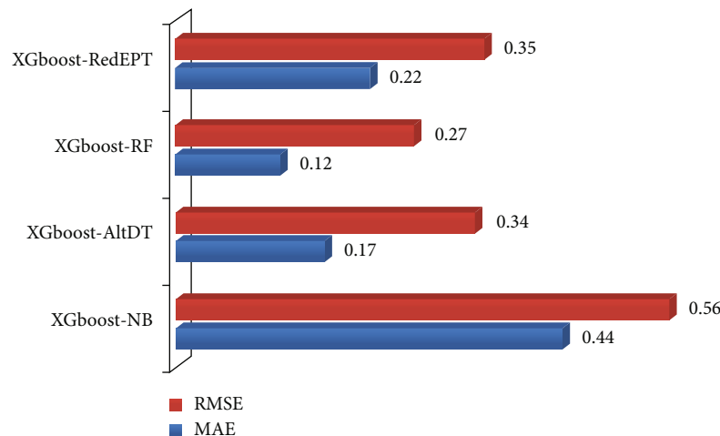
FIGURE 5: Different error rates of XGBoost ensemble classifiers.
