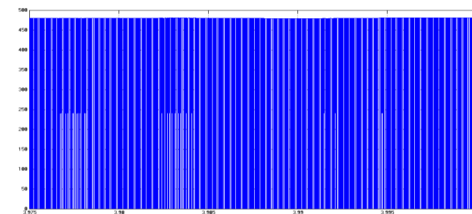
Fig.12. Peak dc Link voltage across inverter Bridge = 480V
