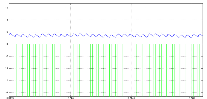
Fig. 15 Diode voltage and inductor current
