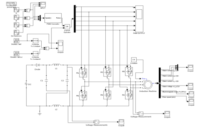
Fig. 9 Simulation configuration
