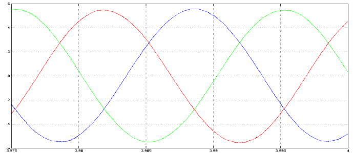
Fig. 13 Three phase stator current
