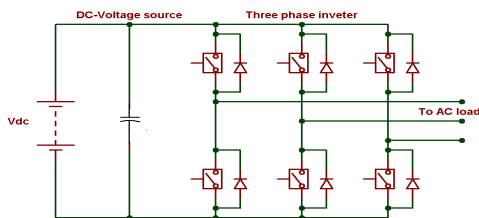
Fig. 1 Traditional voltage source inverter
