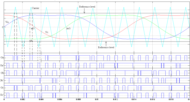
Fig. 8 Maximum constant boost control with third harmonic injection- PWM waveform
