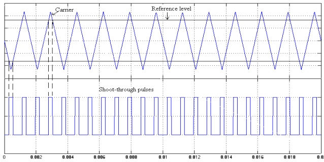
Fig. 7 Shoot-through pulses
