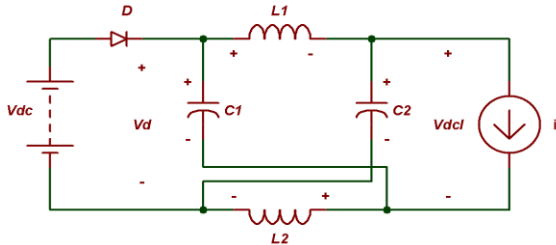
Fig. 4 Equivalent circuit of Z-Source inverter with inverter in active state
