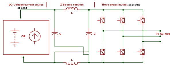
Fig. 3 Z-Source inverter structure
