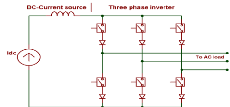
Fig. 2 Traditional current source inverter
