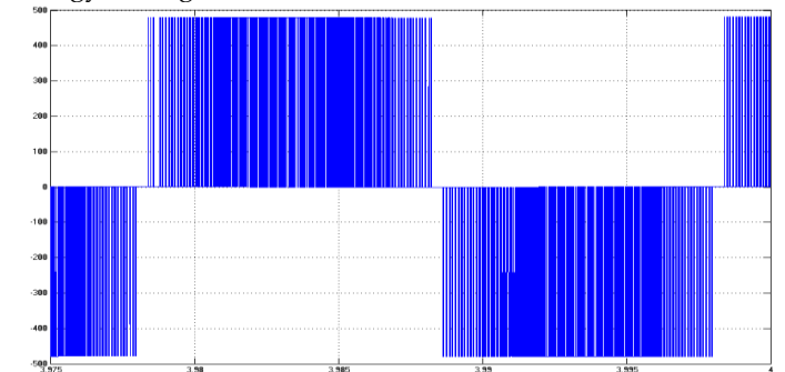
Fig. 14 line to line stator voltage
