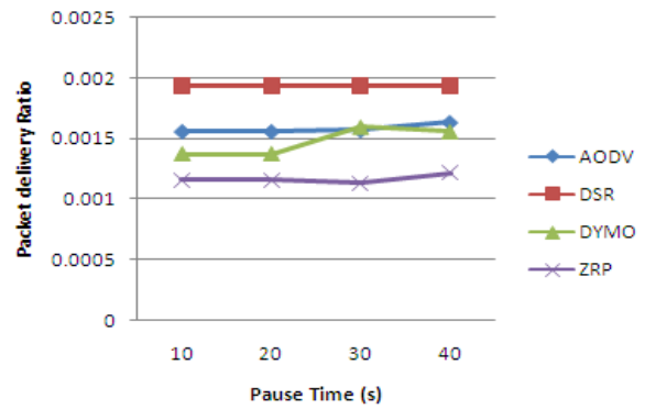
Fig 4: Packet Delivery Ratio (PDR) Vs Pause Time
