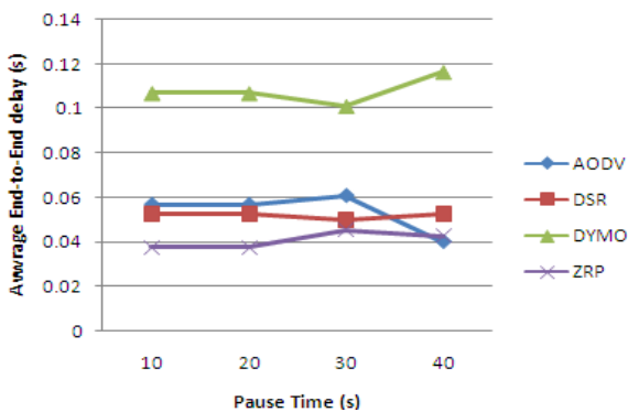
Fig 3: Average End-to-End Delay Vs Pause Time
