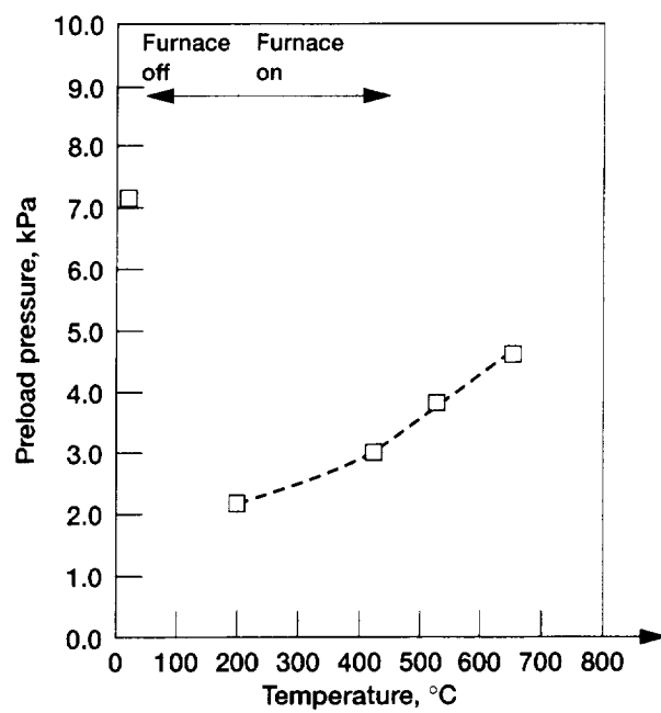
Figure 14.—The effects of bearing temperature on the calculated bearing preload pressure.
