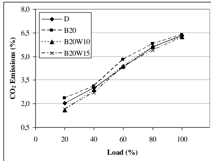
Fig. 7 CO 2 emissions
